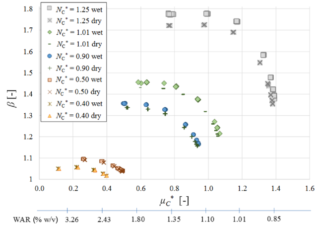
Fig. 6 Steady-state compressor map: static-to-static pressure ratio
