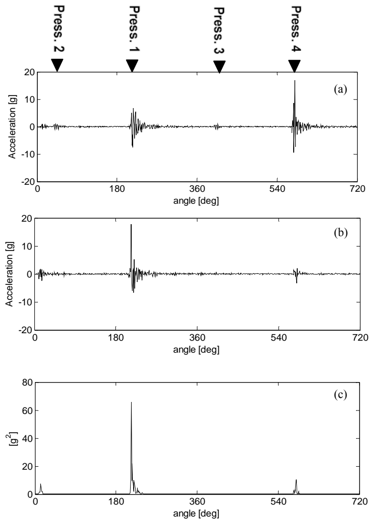
Figure 4. IP1 engine: (a) Time Synchronous Average, (b) residual signal (5 th cycle), (c) Mean Instantaneous Power of the residual signal.
