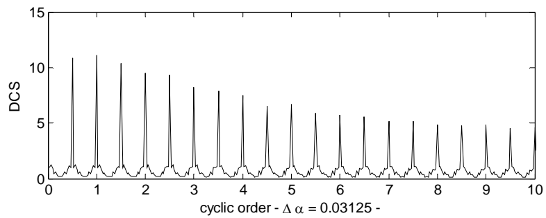
Figure 8. RS4 engine: DCS plotted in the cyclic order range 0-10.
