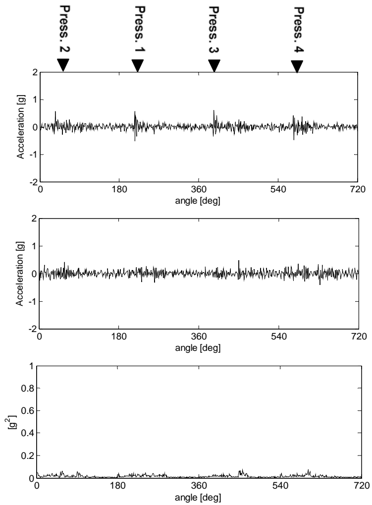
Figure 2. Healthy engine: (a) time synchronous average, (b) residual signal (5 th cycle), (c) Mean Instantaneous Power of the residual signal.
