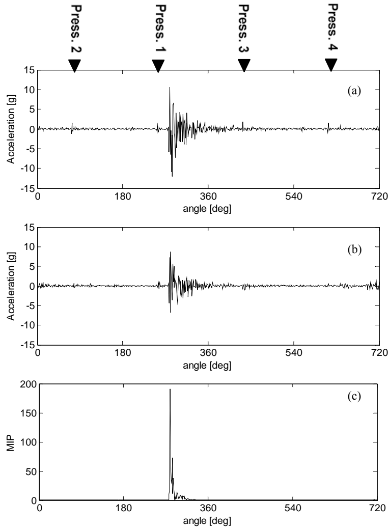
Figure 7. RS4 engine: (a) Time Synchronous Average, (b) residual signal (5 th cycle), (c) Mean Instantaneous Power of the residual signal.
