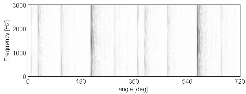
Figure 6. IP1 engine: Wigner Ville Spectrum of the residual signal.
