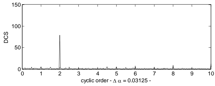
Figure 3. Healthy engine: DCS plotted in the cyclic order range 0-10.
