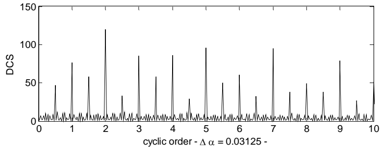
Figure 5. IP1 engine: DCS plotted in the cyclic order range 0-10.
