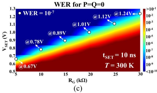
Fig. 6. Simulation results at T = 300 K for READ ( t_{READ} = 10 ns) and SET ( t_{SET} = 10 ns) operations by varying R_G , V_{READ} , and V_{SET} : (a) average read disturbance rate (RDR), (b) average bit error rate (BER) evaluated at V_{REF} \pm 5 mV, (c) write error rate (WER) for the case P=Q=0 .
