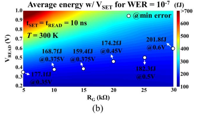
Fig. 7. Simulation results at T = 300 K in terms of (a) average error and (b) average energy consumption (including the contribution of the comparator) by varying R_G and V_{READ} with t_{READ} = t_{SET} = 10 ns and V_{SET} to ensure a WER = 10^{-7} .
