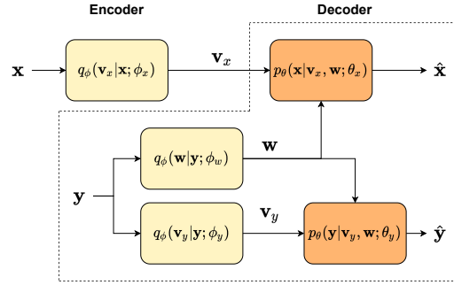
Figure 3: DSC architecture.
