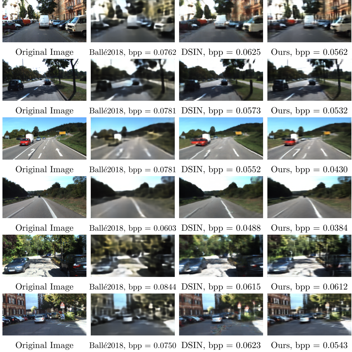
Figure 11: Additional visual comparison of different models from KITTI Stereo dataset in a low bpp range. The models are trained using MS-SSIM distortion function. Notice that in some examples, such as rows 3, 4, and 6, the DSIN model adds some fracture-like effects to the reconstructed image.
