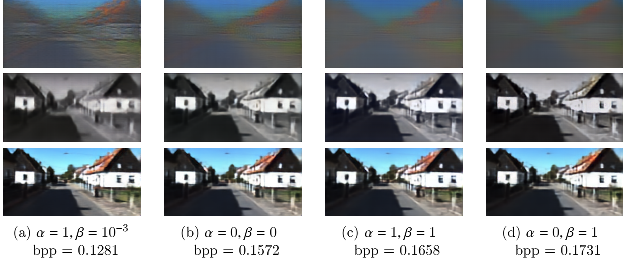
Figure 7: Ablation study: Effect of hyperparameters \alpha and \beta on the common information (1 st row) and private information (2 nd row) decomposition, for a similar reconstruction quality (3 rd row).
