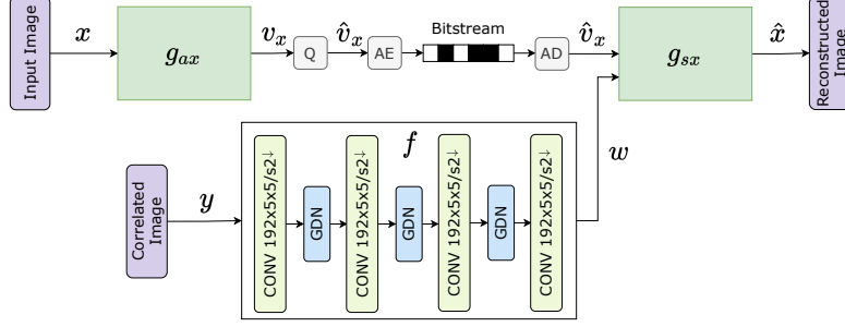
Figure 1: The proposed network architecture for distributed source coding. Block Q corresponds to a uniform quantizer, while blocks AE and AD correspond to arithmetic encoder and arithmetic decoder, respectively.
