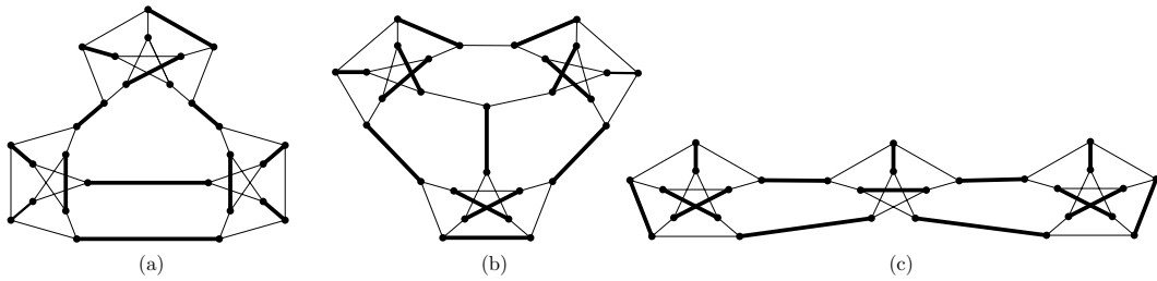
Figure 15: The smallest snarks of oddness 4.
