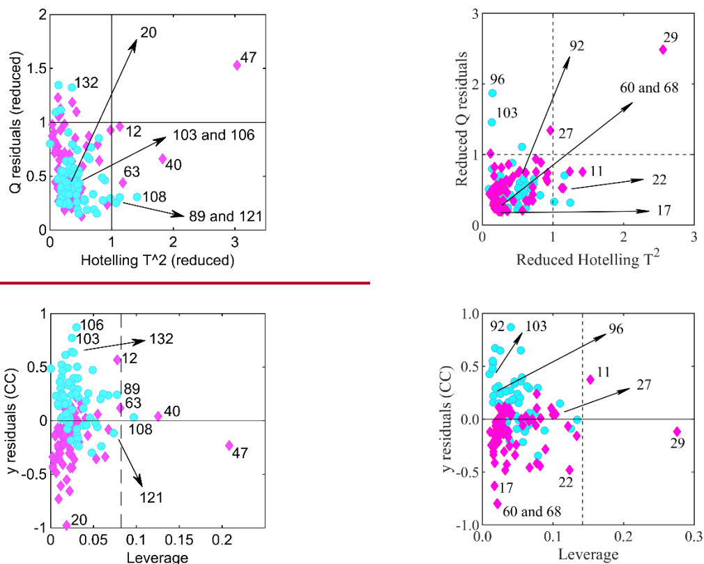
Figure 4. Reduced squared residuals Q vs. reduced Hotelling's T^2 plot, the dashed horizontal and vertical lines show the amplitude of the 95% confidence interval for both parameters (top). Residuals of CC samples vs. leverage plot, the dashed vertical line shows the leverage limit (bottom). Samples are marked according to their class (empty magenta diamonds: cocrystals; black-cyan circles: binary mixtures).
