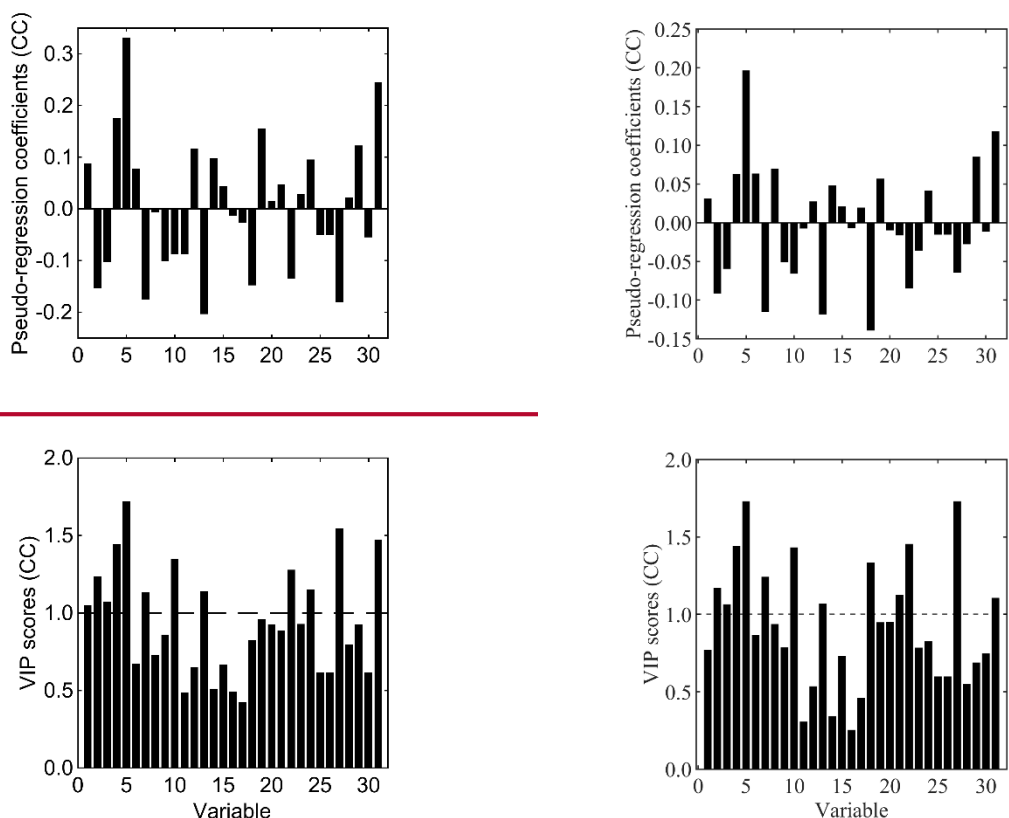
Figure 5. Pseudo-regression coefficients plot for the CC class (top). VIP scores related to each variable included in the X_{cal} space for the CC class, the significance threshold of 1 is depicted as a dashed horizontal line (bottom). Both plots report the variable identification number on the x axis.
