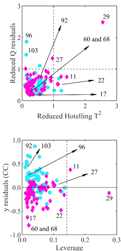
Figure 4. Reduced squared residuals Q vs. reduced Hotelling's T^2 plot, the dashed horizontal and vertical lines show the amplitude of the 95% confidence interval for both parameters (top). Residuals of CC samples vs. leverage plot, the dashed vertical line shows the leverage limit (bottom). Samples are marked according to their class (magenta diamonds: cococrystals; cyan circles: binary mixtures).
