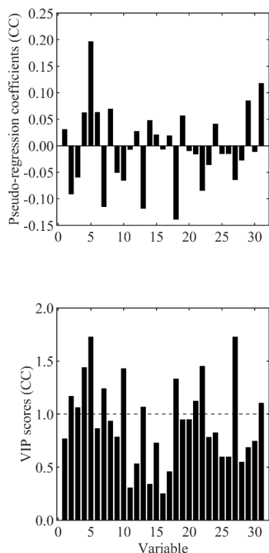
Figure 5. Pseudo-regression coefficients plot for the CC class (top). VIP scores related to each variable included in the X_{cal} space for the CC class, the significance threshold of 1 is depicted as a dashed horizontal line (bottom). Both plots report the variable identification number on the x axis.
