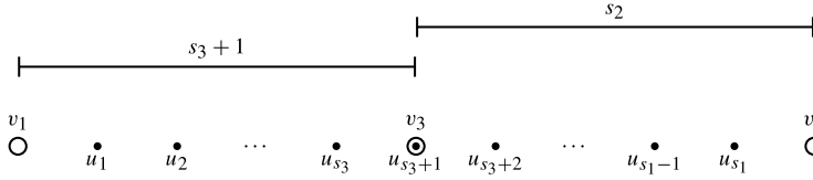
Fig. 6.2. The invariant |\Psi_{3,1}\rangle gives rise to a real string of s_1 uniformly spaced Bethe roots u_k in the complex plane, see (6.35). They lie in between the inhomogeneities v_1, v_2 and one root coincides with v_3 .
