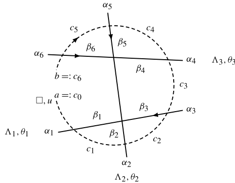
Fig. 3.2. The Baxter lattice introduced in the example of Fig. 3.1 after the dotted circle has been replaced by a dashed auxiliary space line in the fundamental representation \square with spectral parameter u and states labeled a, b at the endpoints. The indices c_i are assigned to the edges of this auxiliary space. The states at the edges connecting this space with the Baxter lattice are labeled \beta_i .
