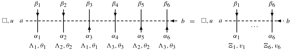
Fig. 3.4. Rewriting of the summed Boltzmann weights in \mathcal{M}_{ab}(u, \mathbf{G}, \mathbf{\Lambda}, \boldsymbol{\theta}, \boldsymbol{\alpha}, \boldsymbol{\beta}) on the l.h.s. as a matrix element \langle \boldsymbol{\alpha} | M_{ba}(u) | \boldsymbol{\beta} \rangle of a monodromy on the r.h.s. for the example discussed in Fig. 3.3. After applying (3.15) to the l.h.s. all vertical lines have the same orientation. \Xi_i and v_i of the resulting monodromy are given by (3.18) with \mathbf{G} specified in the caption of Fig. 3.1.
