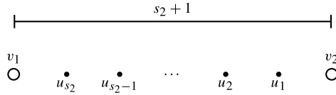
Fig. 6.1. The Bethe roots u_k associated with the Yangian invariant |\Psi_{2,1}\rangle of Section 4.2.1 arrange into a string between the two inhomogeneities v_1 and v_2 , cf. (6.29) in the complex plane. This string consists of s_2 roots with a uniform real spacing of 1.
