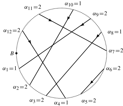
Fig. 2.2. The sample Baxter lattice of Fig. 2.1 with a certain assignment of states, labeled by \alpha , to the endpoints. Note that the number of endpoints i_k with a state labeled \alpha_{i_k} = 1 and that of endpoints j_k with \alpha_{j_k} = 1 agrees, i.e. the ice rule (2.6) is satisfied. In this case \alpha gives rise to \mathbf{x} = (1, 4, 6, 9, 11, 12) , see (2.12), which is used to express the partition function \mathcal{Z}(\mathbf{G}, \theta, \alpha) in terms of a Bethe wave function \Phi(\mathbf{w}, \mathbf{u}, \mathbf{x}) in (2.14).
