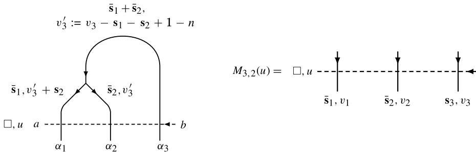
Fig. 4.3. The l.h.s. M_{3,2}(u)|\Psi_{3,2}\rangle of (3.30) for |\Psi_{3,2}\rangle corresponds to the lattice in the left part. It consists of an extended Baxter lattice in form of a trivalent vertex and a dashed auxiliary space. The Boltzmann weights containing the auxiliary space can be formulated as elements of a monodromy M_{3,2}(u) using the crossing relation (3.15) with (4.11). This monodromy is shown in the right part and the parameters of the monodromy obey the constraints (4.29).
