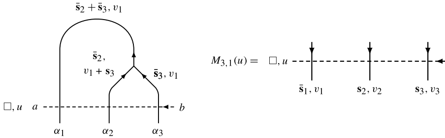
Fig. 4.2. The left part corresponds to the l.h.s. of (3.30) for |\Psi_{3,1}\rangle , i.e. M_{3,1}(u)|\Psi_{3,1}\rangle . It contains a (solid) trivalent vertex, which is an extension of the usual Baxter lattice, and a dashed auxiliary line. Using the crossing relation (3.15) and the crossing parameters in (4.11), the Boltzmann weights involving the auxiliary line can be reformulated as elements of the monodromy M_{3,1}(u) , as is shown on the right side. The necessary constraints on the representation labels and inhomogeneities of the monodromy may be found in (4.23).
