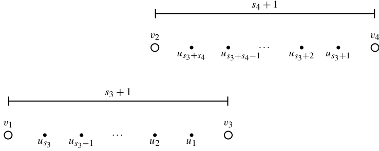
Fig. 6.4. The Bethe roots u_k corresponding to the four site invariant |\Psi_{4,2}(z)\rangle , i.e. to the R -matrix R_{s_3 s_4}(z) , arrange into two real strings in the complex plane. The strings consist of s_3 and s_4 roots, respectively. The difference of their endpoints z := v_3 - v_4 , cf. (4.39), is the spectral parameter of the R -matrix.
