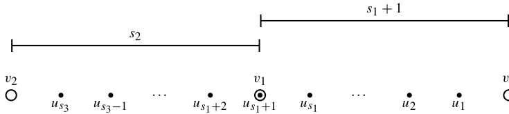
Fig. 6.3. The string of Bethe roots u_k belonging to the invariant |\Psi_{3,2}\rangle . The roots lie between the inhomogeneities v_2 and v_3 . One of them coincides with v_1 .
