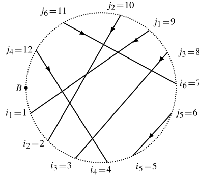
Fig. 2.1. Sample Baxter lattice with N = 6 lines whose configuration is given by the endpoints \mathbf{G} = ((1, 9), (2, 10), (3, 8), (4, 12), (5, 6), (7, 11)) . Each line k has endpoints (i_k, j_k) , an orientation indicated by an arrow and carries a rapidity \theta_k , which is not shown in this figure.
