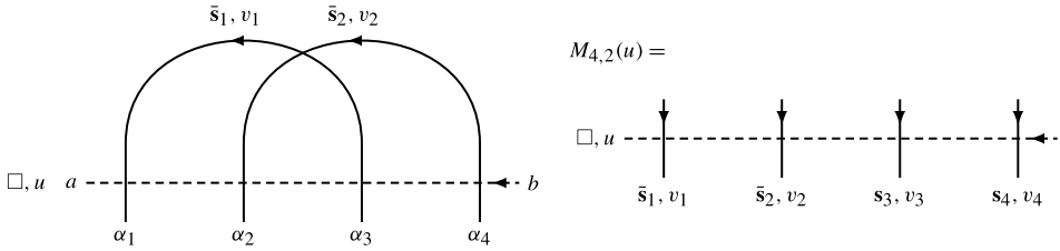
Fig. 4.4. The left part shows a Baxter lattice with two lines specified by \mathbf{G} = ((1, 3), (2, 4)) , \mathbf{A} = (\bar{s}_1, \bar{s}_2) , \theta = (v_1, v_2) , \alpha = (\alpha_1, \alpha_2, \alpha_3, \alpha_4) and a dashed auxiliary space. It corresponds to M_{4,2}(u)|\Psi_{4,2}\rangle as the l.h.s. of (3.30). The right part contains the monodromy M_{4,2}(u) , which is associated with this Baxter lattice. The necessary identifications of the representation labels and the inhomogeneities are written in (4.35).
