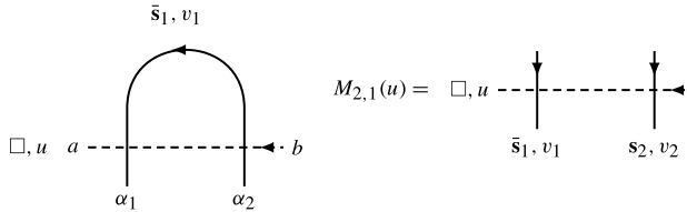
Fig. 4.1. A Baxter lattice with one line specified by \mathbf{G} = ((1, 2)) , \mathbf{A} = (\bar{s}_1) , \boldsymbol{\theta} = (v_1) , \boldsymbol{\alpha} = (\alpha_1, \alpha_2) , cf. (3.1), and intersected by a dashed auxiliary space, left part. This arrangement of Boltzmann weights corresponds to the l.h.s. of the invariance condition (3.30) for |\Psi_{2,1}\rangle , i.e. to M_{2,1}(u)|\Psi_{2,1}\rangle . The elements of the monodromy M_{2,1}(u) in the right part of the figure are obtained from the Boltzmann weights on the left side using the crossing relation (3.15). The representation labels and inhomogeneities of this monodromy obey (4.17).
