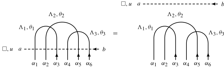
Fig. 3.3. An identity for \mathcal{Z}(\mathbf{G}, \mathbf{A}, \boldsymbol{\theta}, \boldsymbol{\alpha}) of the sample Baxter lattice in Fig. 3.1 is derived by disentangling the dashed auxiliary line from the solid lines using (3.7) and (3.8). The lattice has been deformed to emphasize that the row of vertices involving the auxiliary line will be written as a monodromy shortly, cf. Fig. 3.4.
