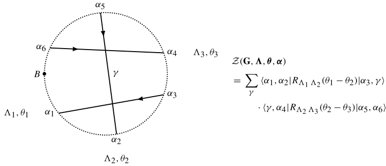
Fig. 3.1. Example of a (generalized) Baxter lattice with N = 3 lines and \mathbf{G} = ((1, 3), (2, 5), (4, 6)) , left side. Each line carries a \mathfrak{gl}(n) representation \Lambda_k , a spectral parameter \theta_k , two state labels \alpha_{i_k} and \alpha_{j_k} at the endpoints i_k < j_k and an orientation indicated by an arrow. The dotted circle and the reference point B are not part of the Baxter lattice. The associated partition function \mathcal{Z}(\mathbf{G}, \mathbf{\Lambda}, \boldsymbol{\theta}, \boldsymbol{\alpha}) is shown on the right, cf. (3.6).
