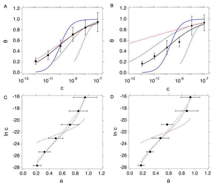
Fig. 3. Top: \theta vs c plots for OECT (A) and EGOFET (B). Continuous blue and black lines are fit to the Langmuir (eq. 1a) and Hill (eq. 2a) isotherms. Dotted blue, black and red lines are fit of the c vs \theta plot to the Langmuir (eq. 1b), Hill (eq. 2b) and Frumkin (eq. 3) isotherms. Bottom: \ln c vs \theta plots for OECT (C) and EGOFET (D). Dashed blue, black and red lines are fit to the Langmuir, Hill and Frumkin isotherms. Error bars represent the associated standard error of the mean SEM.
