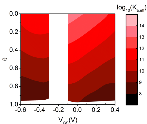
Fig. 5. Contour plot of the effective binding constant as \text{Log}_{10} (K_{a,eff}) as a function of \theta and V_{GS} for EGOFET (left strip) and OECT (right strip).
