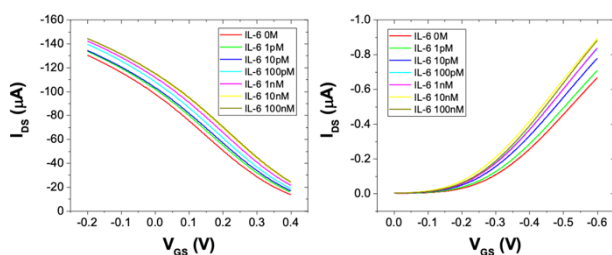
Fig. 2. Overlay of transfer characteristics for an OECT (A) and an EGOFET (B) upon incubation with different concentrations of IL-6, at V_{DS} = -0.2 V.
