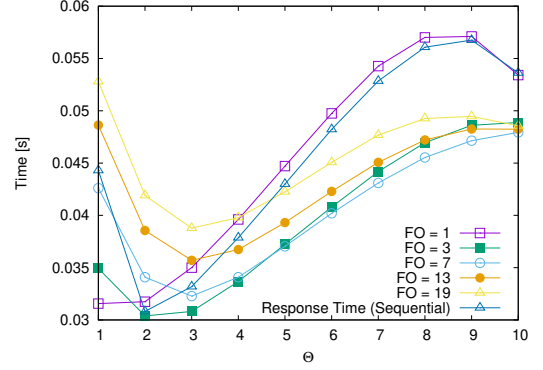
Figure 6: Response time for different Fan-out FO
