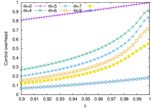
Figure 1: Control overhead vs loads.
