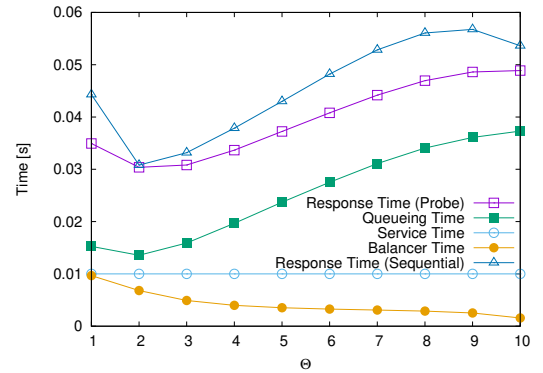
Figure 4: Response time vs. Threshold \Theta ( FO = 3 )
