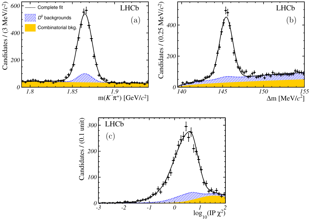
Fig. 2. Mass and \log_{10}(\text{IP } \chi^2) distributions for selected D^{*+} \rightarrow D^0(K^-\pi^+)\pi^+ candidates showing (a) the masses of the D^0 candidates for a window of \pm 1.6 \text{ MeV}/c^2 (approximately \pm 2\sigma ) around the fitted \Delta m peak, (b) the differences between the D^{*+} and D^0 candidate masses for a mass window of \pm 16 \text{ MeV}/c^2 (approximately \pm 2\sigma ) around the fitted m(K^-\pi^+) peak, and (c) the \log_{10}(\text{IP } \chi^2) distribution of the D^0 candidate for a mass signal box of \pm 16 \text{ MeV}/c^2 around the fitted m(K^-\pi^+) peak and \pm 1.6 \text{ MeV}/c^2 around the fitted \Delta m peak. Projections of a likelihood fit to the full data sample are shown with components as indicated in the legend. The ‘ D^0 backgrounds’ component is the sum of the secondary, prompt random slow pion, and secondary random slow pion backgrounds.
