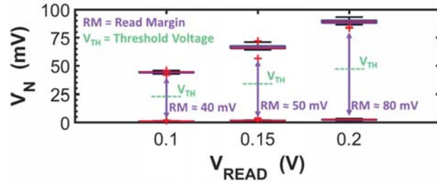
Fig. 5. Distribution of V_N calculated at different V_{\text{READ}} , including the effect of variability and RTN over 50 cycles. The upper and lower boxes represent the cases P \neq Q and P = Q = 0 , respectively, showing the medians (red lines), the 25 th to 75 th percentiles extension (blue boxes), and the most extreme data points (black whiskers). The red crosses represent the worst-case fluctuations due to RTN. The read margins (RMs – violet arrows) and associated threshold voltages ( V_{\text{TH}} – ocean green dashed lines) for the comparator are shown.
