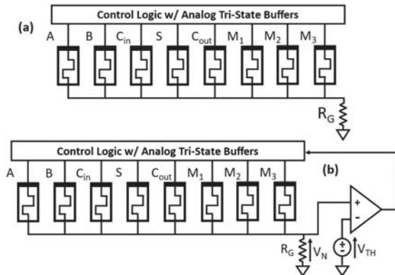
Fig. 8. 1-bit full-adder implementation using (a) the IMPLY and (b) the SIMPLY architectures.
