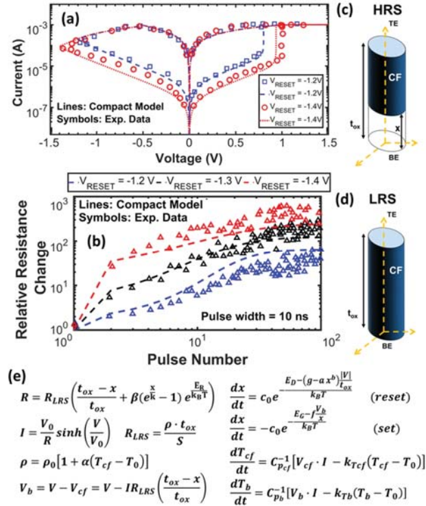
Fig. 1. (a) Simulated (lines) and experimental (symbols) DC I-V curves of a multilayer TiOx/HfOx RRAM device during set and reset operations in different reset conditions (i.e., V_{\text{RESET}} = -1.2 V, and -1.4 V, with different colors). Data from [18]. (b) Simulated (lines) and experimental (symbols) pulsed reset curves using a train of 10 ns pulses with different voltages (i.e., V_{\text{RESET}} = -1.2 V, -1.3 V, and -1.4 V, with different colors). Data from [18]. (c-d) Sketch of the compact model of a device in HRS (c) and LRS (d). (e) The compact model equations, where R is the total device resistance, R_{\text{LRS}} the value of R in LRS, t_{\text{ox}} the oxide thickness (12 nm in this case), x the barrier thickness, k the typical tunneling length, T the device temperature, T_0 the ambient temperature, k_B the Boltzmann constant, I the current, V the applied voltage, S the filament cross-section, \rho its resistivity. E_R , E_D , E_G , g , f , c_0 , a , b , \beta , k_{\text{Tcf}} , k_{\text{Tb}} , C_{\text{pof}} and C_{\text{pb}} are material-related constants for defect diffusion and generation, and for thermal dissipation [10, 16–17].
