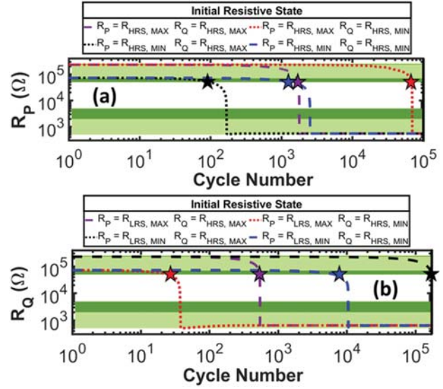
Fig. 3. Degradation of R_P over time during the repeated execution of the IMPLY operation with P=Q=0 . Four corner cases are considered to account for variability ( R_P is initialized either at R_{HRS,MIN} or at R_{HRS,MAX} and R_Q is kept fixed either at R_{HRS,MIN} or at R_{HRS,MAX} ). The degradation depends on the initial values of R_Q and R_P , resulting in errors (star symbols) potentially after \sim 100 cycles (black star). (b) Degradation of R_Q over time during the repeated execution of the IMPLY operation with P=1 and Q=0 . Four corner cases are considered to account for variability ( R_P is initialized either at R_{LRS,MIN} or at R_{LRS,MAX} and R_Q is initialized either at R_{HRS,MIN} or at R_{HRS,MAX} ). In the worst case, the degradation of R_Q results in errors after \sim 30 cycles (red star).
