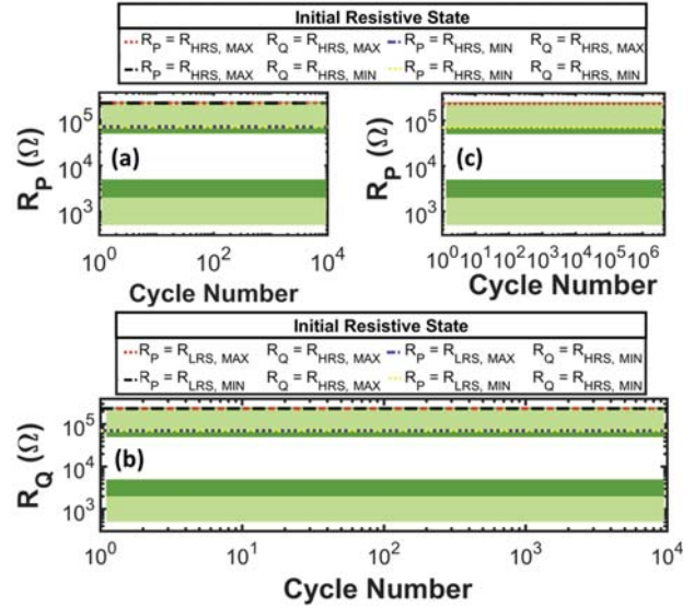
Fig. 7. Benefits of using SIMPLY. (a) R_P vs. cycle number during the repeated execution of the IMPLY operation with P=Q=0 and V_{\text{READ}}=200\text{mV} . The same four corner cases as in Fig. 3(a) are considered to account for variability. No degradation is observed up to 10^4 cycles. (b) R_Q vs. cycle number during the repeated execution of the SIMPLY operation with P=1 and Q=0 . The same four corner cases as in Fig. 3(b) are considered to account for variability. No degradation is observed up to 10^4 cycles. (c) No degradation up to 4.5 \cdot 10^6 cycles occurs for the two worst cases, i.e., P=Q=0 with initial R_P=R_Q=R_{\text{HRS,MAX}} (maximum voltage drop across P and Q) and R_P=R_Q=R_{\text{HRS,MIN}} (maximum current on P and Q). In all cases, V_{\text{READ}}=200\text{mV} .
