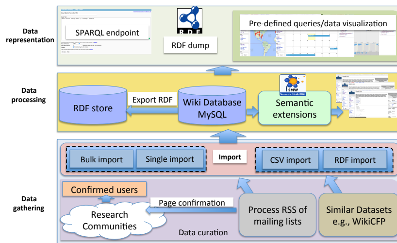
Figure 2: OpenResearch Architecture
