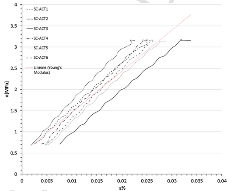
Fig. 12. Stress-strain curves and trend line for the Young modulus.
