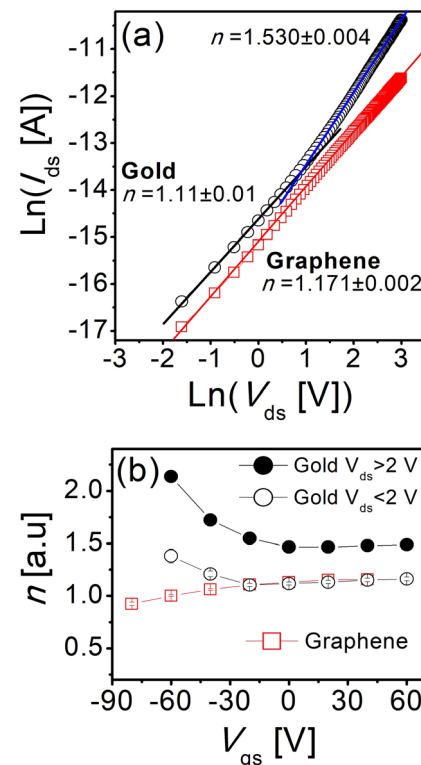
FIG. 3. (a) Ln-Ln plot of the output curves for V_{gs} = +20 V of the graphene-based device (red squares) and for the gold-based transistor (black circles) with L = 140 \pm 30 nm. The n values indicate the slope of the ln-ln curves extracted from the linear best fit. (b) Slopes n extracted as a function of the applied gate-source bias in both the architectures for L = 140 \pm 30 nm. For gold electrode devices, the responses for V_{ds} < 2 V (empty circles) and V_{ds} > 2 V (filled circles) are reported.
