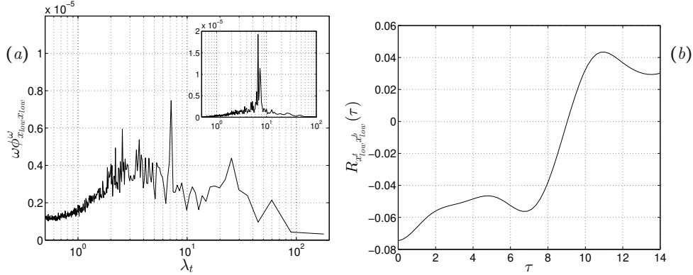
FIGURE 14. (a) Premultiplied frequency spectrum of the streamwise movement of low pressure levels at the wall, \omega \Phi_{x_{low}^t x_{low}^b}^\omega . Inset: premultiplied frequency spectrum of vertical velocity, \omega \Phi_{vv}^\omega , evaluated in the wake at a location corresponding to the point P5 shown in figure 2(a). (b) Correlation function R_{x_{low}^t x_{low}^b}(\tau) , equation (7.3).
