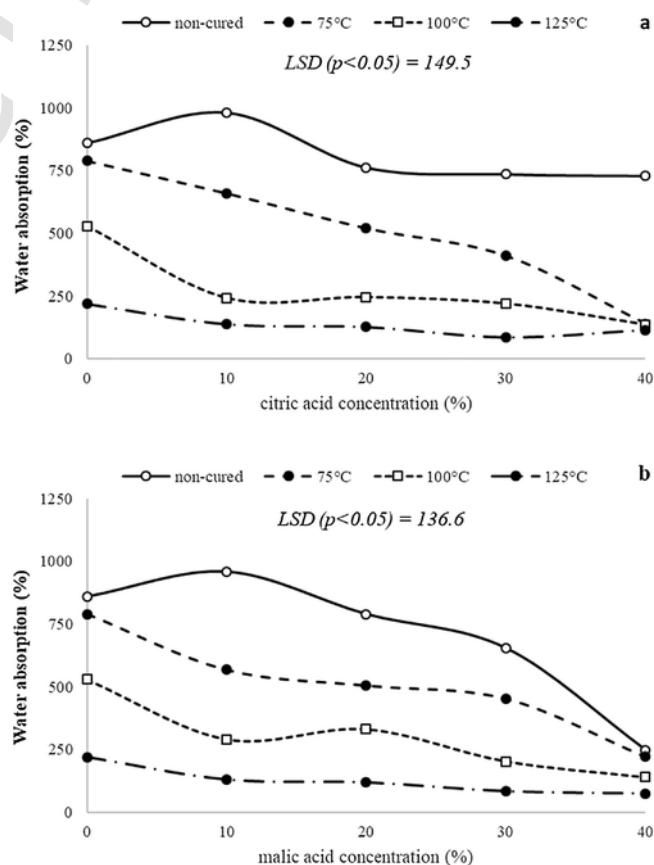
Fig. 4. Effect of citric (a) and malic (b) acid addition on water absorption of PVOH films cured at different temperatures. Significance of difference among means is based on the least significant difference (LSD) for p < 0.05 .
