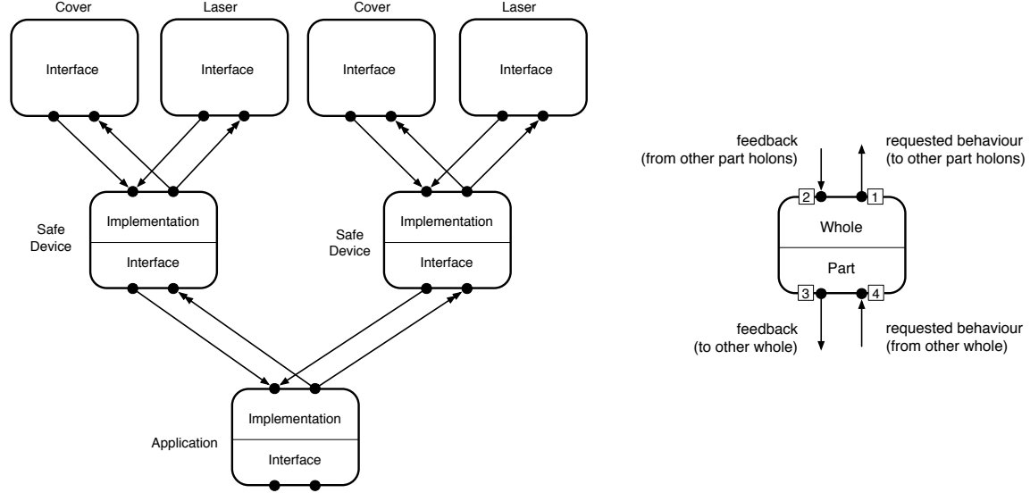
Figure 2: The holarchy of an application built from two instances of the safe device of Figure 1 and the communication ports of a single holon.
