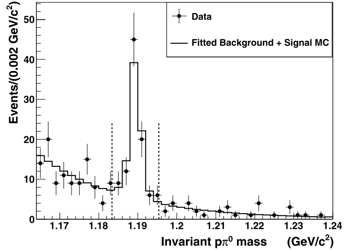
Fig. 1. Reconstructed p\pi^0 invariant mass distribution for \Xi^0 \rightarrow \Sigma^+\mu^-\bar{\nu}_\mu candidates after all selection criteria were applied. Points with error bars are data. The peak at the \Sigma^+ mass value shows clear evidence for the signal. The vertical dashed lines delimit the signal region. The background was evaluated with a likelihood fit of the data performed in two intervals, between 1.164 and 1.180 \text{GeV}/c^2 and between 1.198 and 1.240 \text{GeV}/c^2 . The solid histogram shows the sum of the background contribution (evaluated from the fit) and the Monte Carlo sample of the signal normalized to the events found in the data after background subtraction.
