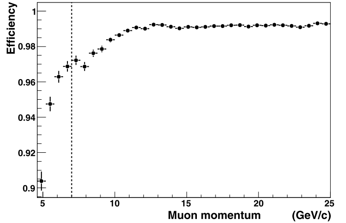
Fig. 2. Efficiency for muon identification as a function of muon momentum (right), the dashed line shows the lower threshold at 7 GeV/c applied to muon momentum.
