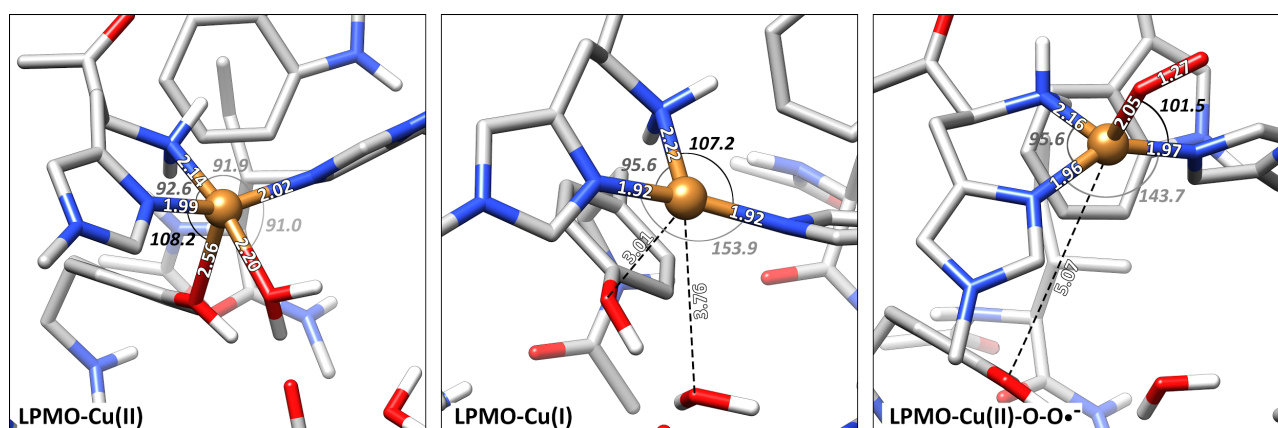
Figure 2: Coordination geometry of the copper ion in the LPMO-Cu(II) ( P OX ), LPMO-Cu(I) ( P RED ) and LPMO-Cu(II)-O-O •- ( P O2 ) species with selected interatomic distances (in angstroms) and angles (in degrees). For the sake of clarity, aliphatic hydrogen atoms are not shown.
