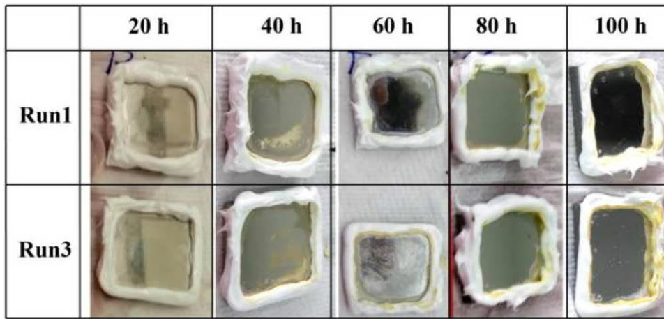
Figure 23. Photographs of samples Run1 and Run3 after each 20 hour-cycle of Corrodkote testing, after removal of the corrosive slurry.
