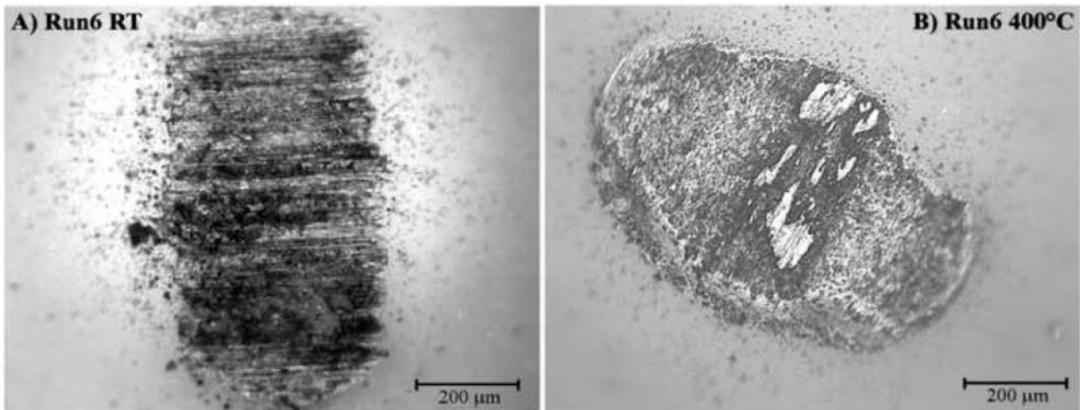
Figure 12. Optical micrographs of \text{Al}_2\text{O}_3 counterparts used against sample Run6 at room temperature (A) and 400°C (B).
