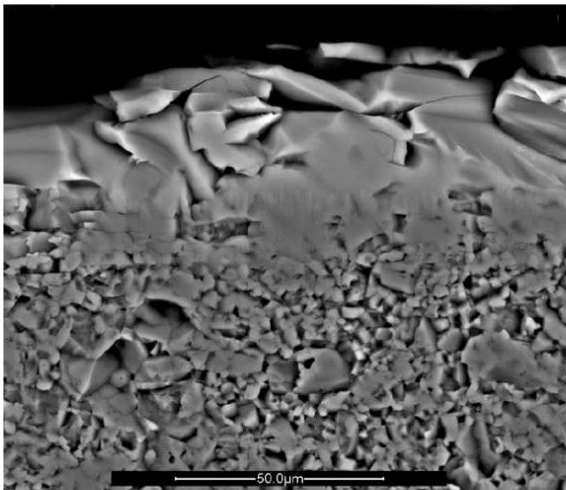
Figure 5 – Example of a bioactive glass-based FGC enameled on alumina. Light gray areas on top: glass; dark gray areas: alumina. Scale bar: 50 \mu\text{m} .
