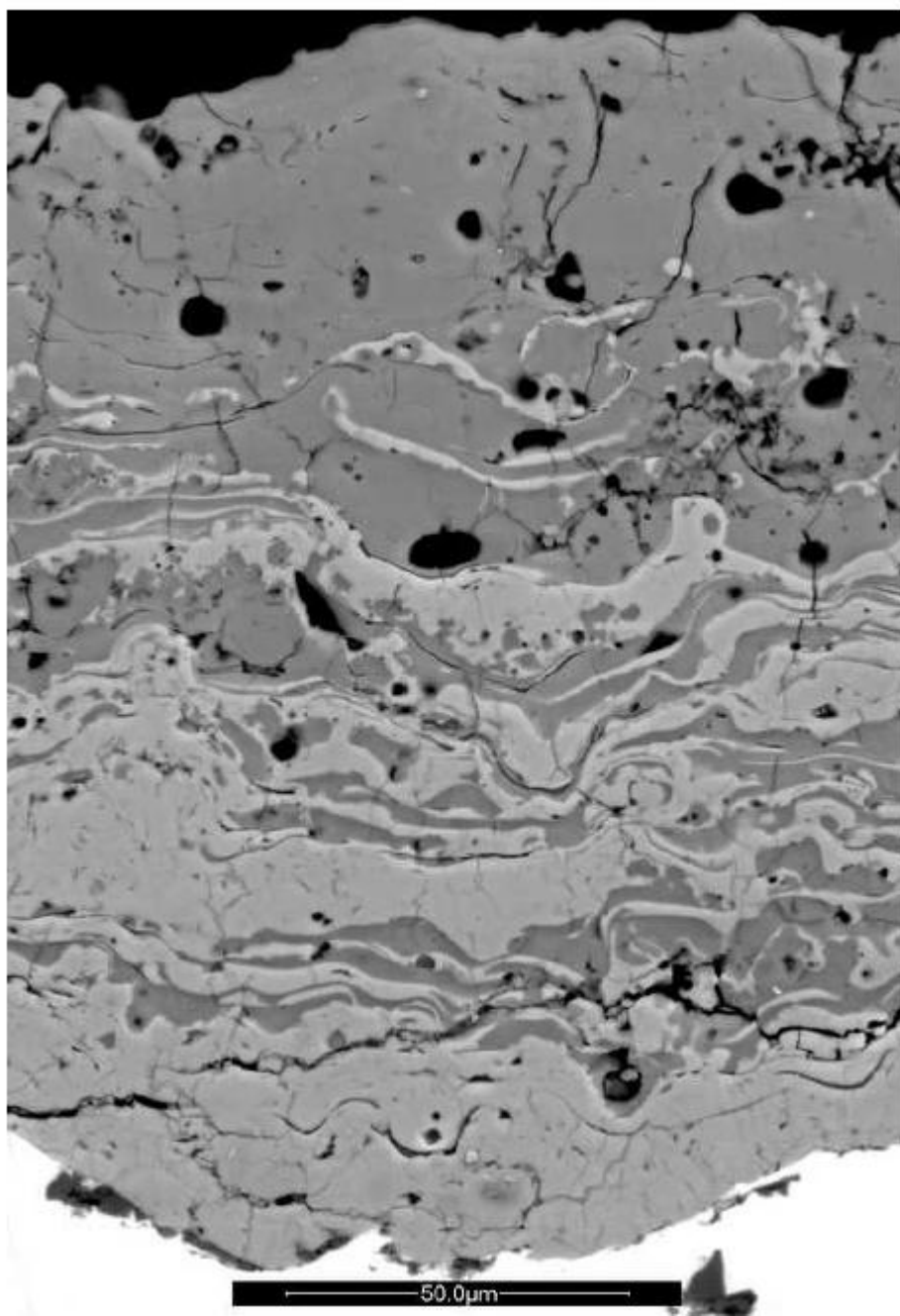
Figure 3 – Example of a titania-HA FGC applied on Ti-6Al-4V by means of air plasma spraying. Dark gray: HA; light gray: titania; white: Ti-6Al-4V substrate. The FGC presents the typical lamellar structure of plasma sprayed deposits. Scale bar: 50 \mu\text{m} .
