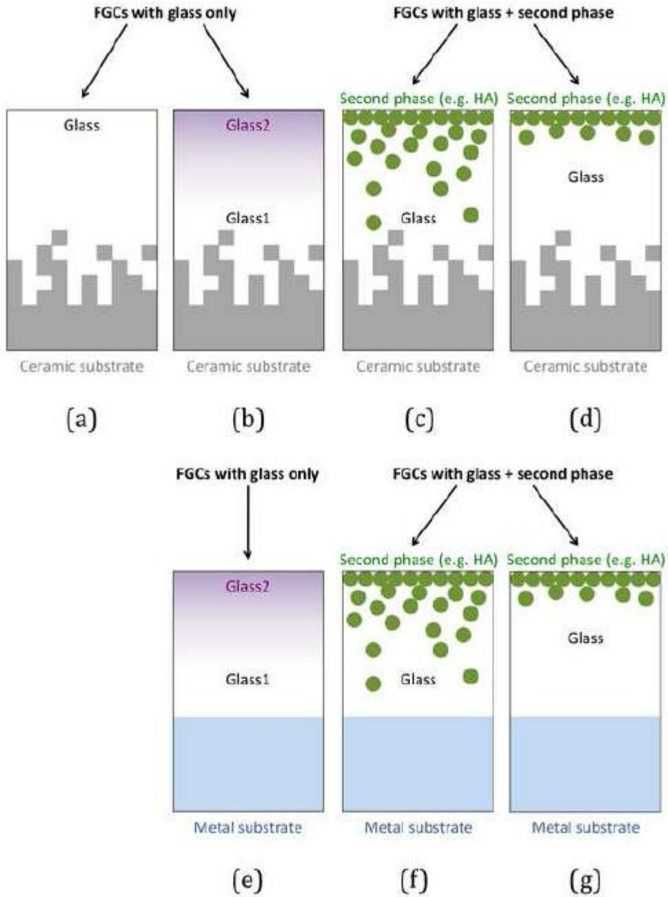
Figure 4 – Basic types of FGCs produced by firing/enameling on ceramic substrates (a-d) and on metal substrates (e-g). In order to obtain a glassy FGC, one glass is enough for ceramic substrates (a, b), whereas at least two glasses are required for metal substrates. As an alternative solution, a second (non glassy) phase can be introduced, thus creating a “composite” FGC (c, d, f, g).
