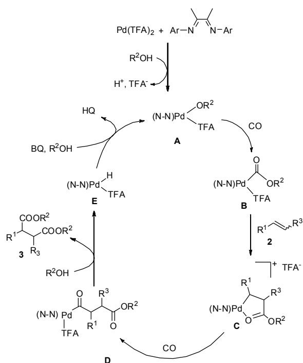
Scheme 3. Proposed catalytic cycle.
