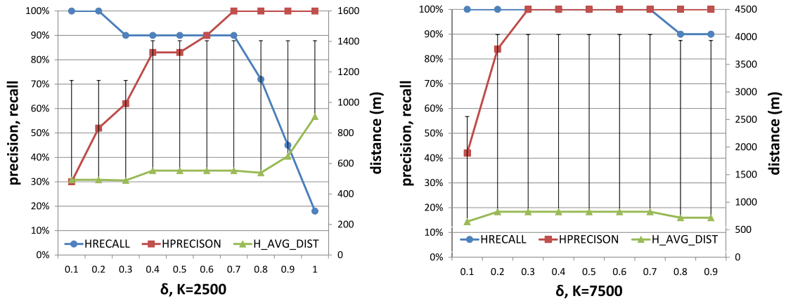
Fig. 4. Results obtained for different values of k and \delta using leave-one-out data as input. Identification of the home place. We report precision, recall and the average distance at which location can be identified.
