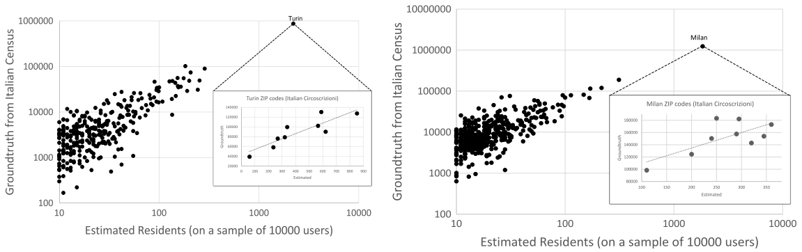
Fig. 8. Correlation between the number of people living in a city as measured by our approach and by the Italian census. (left) Piemonte, (right) Lombardia. Plot details for the city of Turin and Milan.
