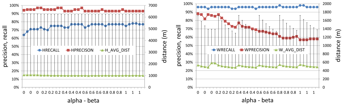
Fig. 5. Results obtained for different values of \alpha and \beta . (left) Identification of the home place. (right) Identification of the work place.
