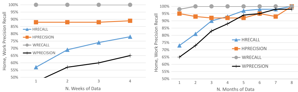
Fig. 6. Recall and precision results for an increasing amount of input data. (left) Results varying the number of weeks provided to the algorithm. (right) Results varying the number of months provided to the algorithm.
