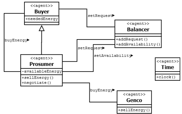
Fig. 3 Agent model
