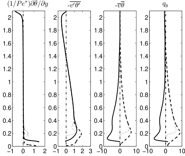
Figure 9: Profiles of the vertical heat fluxes for subsequent axial positions, Pr = 0.71 . Dotted line, x = 0.3 ; dashed line, x = 0.9 ; solid line, x = 1.4 .
