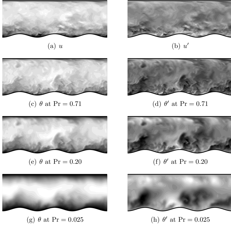
Figure 6: Snapshots of the instantaneous streamwise velocity component and temperature fields: u in a; u' in b, \theta in c,e,g; \theta' in d,f,h.
