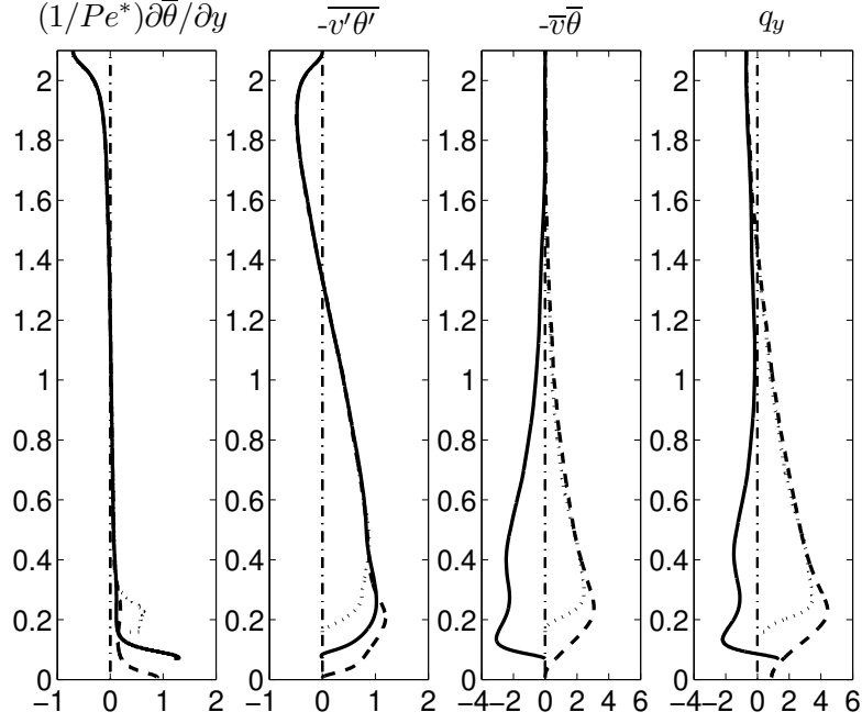
Figure 10: Profiles of the vertical heat fluxes for subsequent axial positions, Pr = 0.20 . Dotted line, x = 0.3 ; dashed line, x = 0.9 ; solid line, x = 1.4 .
