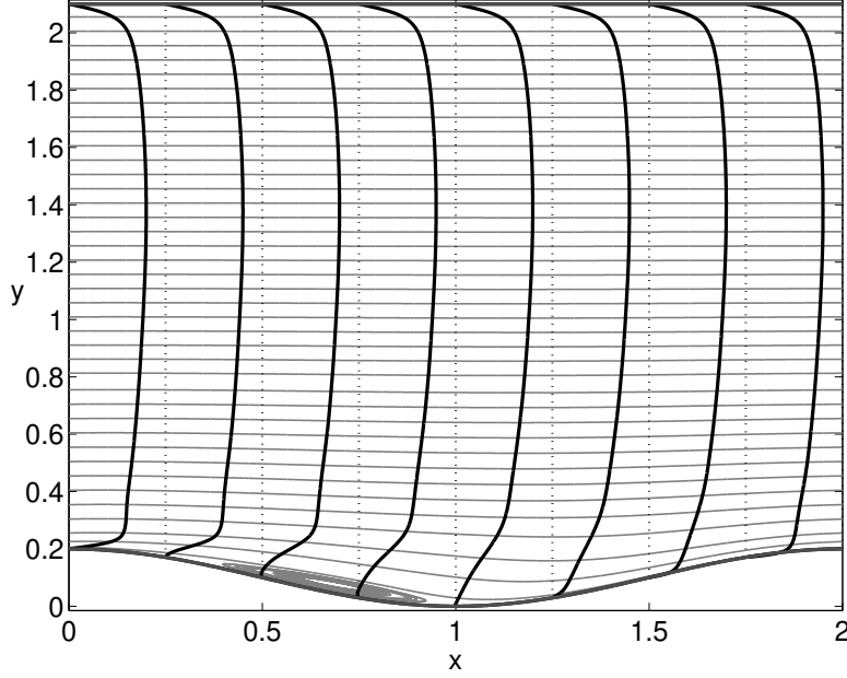
Figure 3: Profiles of the streamwise component of the mean velocity field and streamlines.
