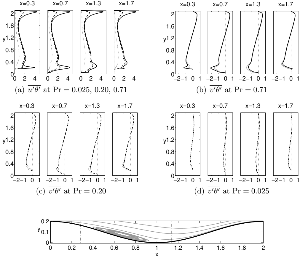
Figure 8: Profiles of turbulent heat fluxes, (a) \overline{u'\theta'} : solid line \text{Pr} = 0.71 ; dashed line \text{Pr} = 0.20 ; dash-dot line \text{Pr} = 0.025 . Insets (b) (c) (d), black lines: vertical heat fluxes; gray lines: heat fluxes calculated on a reference frame locally aligned with the wavy walls.
