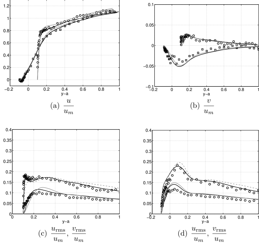
Figure A.18: Validation of the numerical technique employed by comparison with experiments and DNS results from the literature. (a) Profiles of the normalized mean streamwise velocity for crest and trough. Gray lines indicate present results; symbols indicate measurements in Ref. [6]; solid black lines are for the DNS in Ref. [10]. (b) Profiles of the normalized mean vertical velocity for crest and trough. Legend is like for figure A.18a. (c) Profiles of the normalized root-mean-square velocity fluctuations at the crest. The dashed gray line indicates u_{rms}/u_m , the solid gray line is for v_{rms}/u_m ; symbols indicate measurements in Ref. [6]; dashed lines are for the DNS in Ref. [10]. (d) Profiles of the normalized root-mean-square velocity fluctuations at the trough; legend is like for figure A.18c
