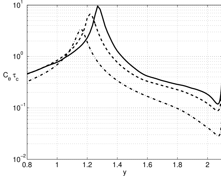
Figure 16: Time, x and z average of the C_\theta \tau_c product for y - y_w \gtrapprox 0.7 and for three different Prandtl number values, solid line: \text{Pr} = 0.71 ; dashed line: \text{Pr} = 0.20 and dash-dot line \text{Pr} = 0.025 .
