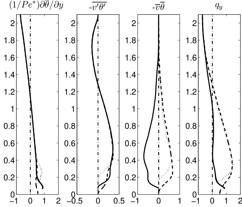
Figure 11: Profiles of the vertical heat fluxes for subsequent axial positions, Pr = 0.025 . Dotted line, x = 0.3 ; dashed line, x = 0.9 ; solid line, x = 1.4 .
