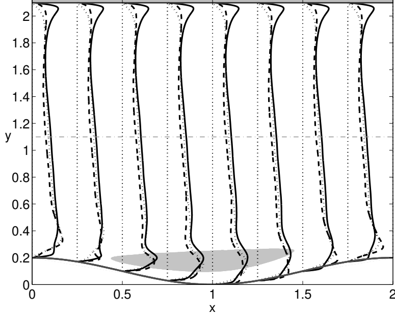
Figure 4: Profiles of the root-mean-square velocity fluctuations. Solid line, u_{\text{rms}} ; dotted line, v_{\text{rms}} ; dashed line, w_{\text{rms}} . The gray area is the region where Reynolds stress -\overline{u'v'} are greater than 2.1. A gray, horizontal, dashed line indicates the channel centerline y = 1.1\delta .
