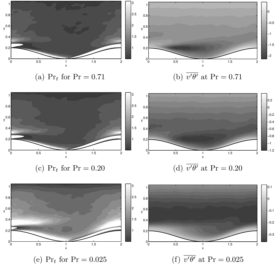
Figure 13: Contour plots of the time-averaged turbulent Prandtl number over the wavy walls are displayed in insets (a), (c), (e). White regions indicate \text{Pr}_t < 0.50 or \text{Pr}_t > 3.3 . Insets (b), (d), (f) display contour plots of the time-averaged vertical heat fluxes. Values of \langle \text{Pr}_t \rangle for the three molecular \text{Pr} are given in table 2.
