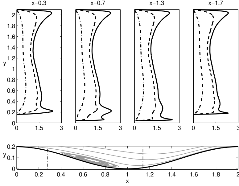
Figure 7: Root-mean-square of the temperature fluctuations, \theta_{\text{rms}} , solid line: \text{Pr} = 0.71 ; dashed line: \text{Pr} = 0.20 and dash-dot line \text{Pr} = 0.025 .
