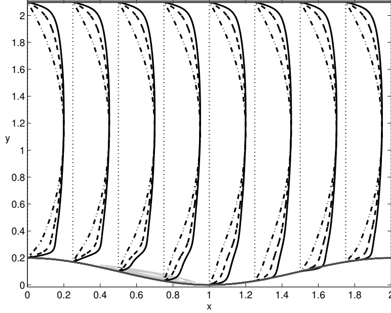
Figure 5: Profiles of the normalized mean temperature field \theta for three different Prandtl number values, solid line: Pr = 0.71 ; dashed line: Pr = 0.20 and dash-dot line Pr = 0.025 . Streamlines of the mean vortex are also indicated in the figure.
