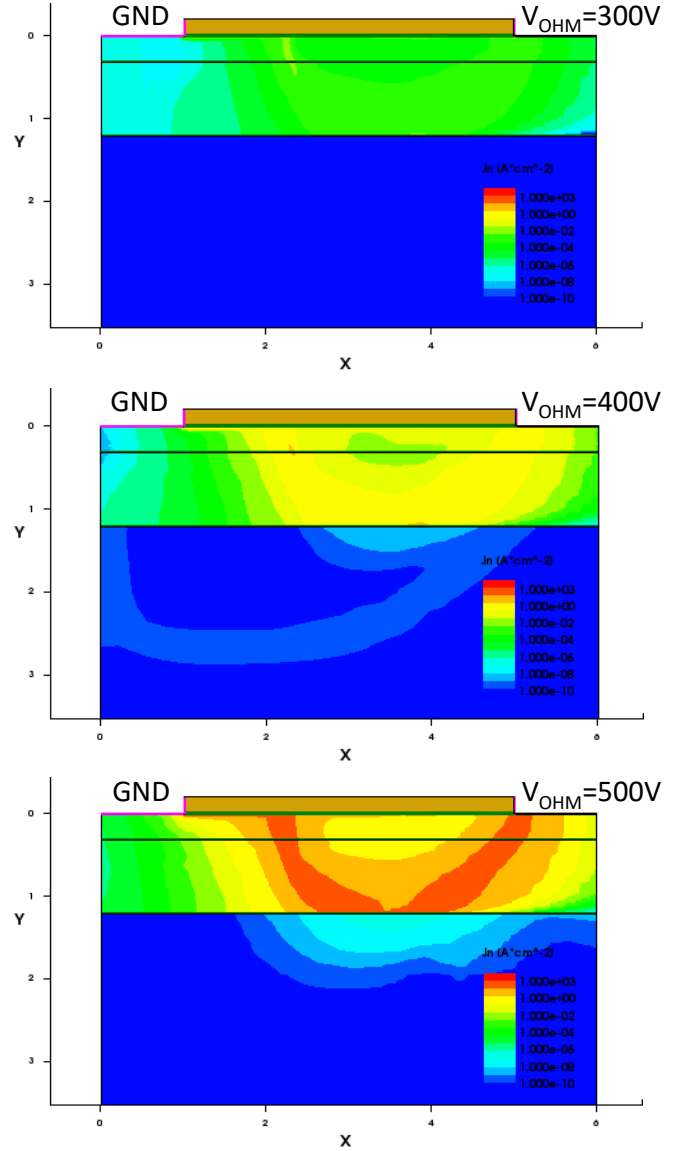
Fig. 3. Simulated electron current density plots in a lateral isolation structure with L_{ISOL} = 1.2 \mu m and a gap of 1.4 \mu m between the isolation implant and the ohmic contacts on both sides. The left ohmic contact and the substrate contact (not shown in these enlarged plots) are grounded, while different positive voltages are applied to the right ohmic contact.
