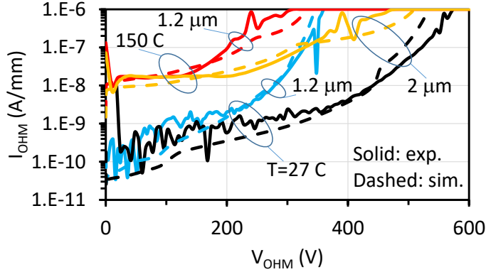
Fig. 2. Experimental (solid) and simulated (dashed) IV curves in lateral, ohmic-to-ohmic isolation structures for two different isolation implant lengths ( L_{ISOL} ) and two different temperatures. Same setup as for Fig. 1.
