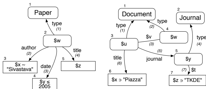
Figure 2: Query 1 (left) and Query 2 (right)
