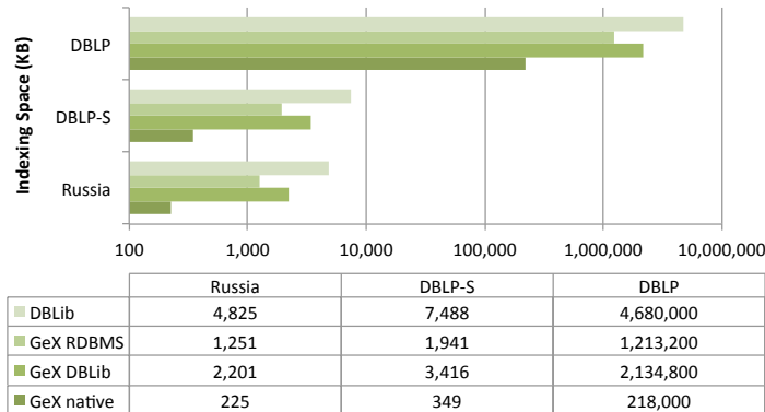
Figure 14: Indexing space comparison between different implementations
