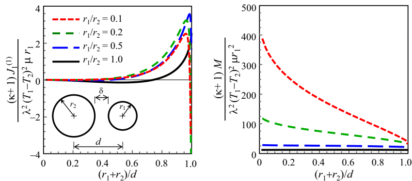
FIGURE 2: Variations of the normalized J_1^{(1)} - and M -integrals with the holes geometry.
