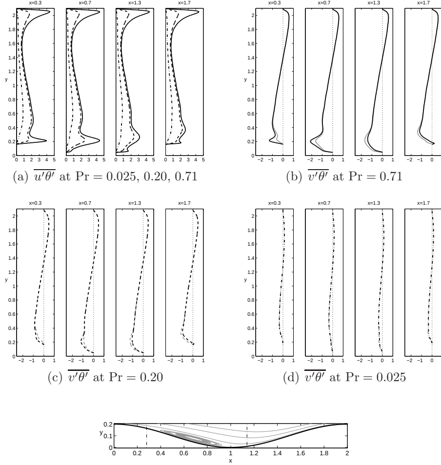
Figure 11: Profiles of turbulent heat fluxes, (a) \overline{u'\theta'} : solid line \text{Pr} = 0.71 ; dashed line \text{Pr} = 0.20 ; dash-dot line \text{Pr} = 0.025 . Insets (b) (c) (d), black lines: vertical heat fluxes; gray lines: heat fluxes calculated on a reference frame locally aligned with the wavy walls.
