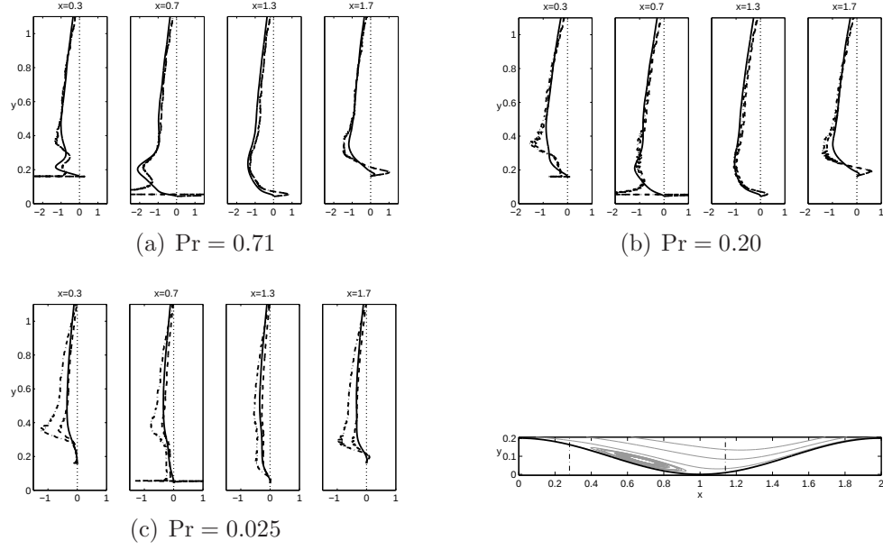
Figure 15: Comparison between turbulent heat fluxes in y direction, for the three different Pr . Solid line: results by DNS; dashed line: results by SGD model with \widehat{Pr}_t as in equation (19); dash-dot line: results by SGD model using \widehat{Pr}_t = 0.9 for all Pr .
