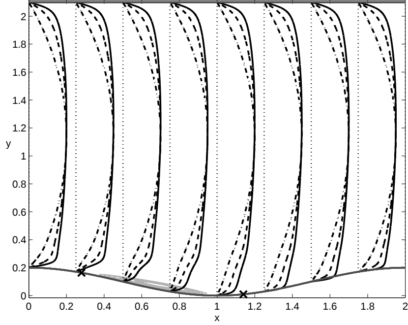
Figure 7: Profiles of the normalized mean temperature field \theta for three different Prandtl numbers, solid line: Pr = 0.71 ; dashed line: Pr = 0.20 and dash-dot line Pr = 0.025 . Mean separation and reattachment locations are indicated by x-symbols. Streamlines of the mean vortex are also indicated in the figure.
