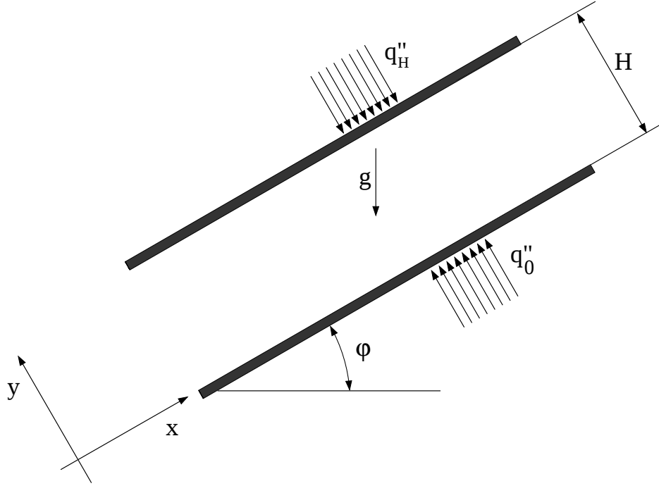
Figure 1: Two-dimensional representation of the inclined channel.
