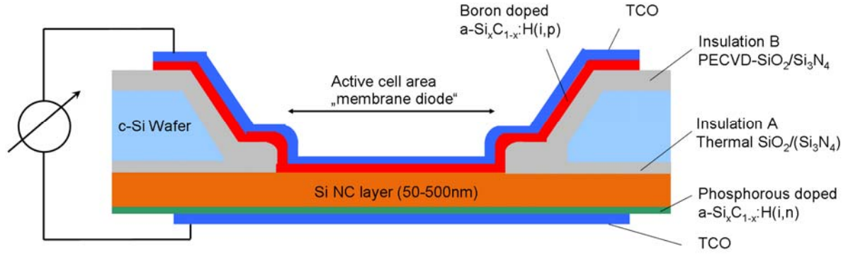
Figure 3. Structure for a vertical p-i-n solar cell with a Si nanocrystal thin film in the intrinsic region and selective electron and hole contacts by doped amorphous silicon carbide ( \text{a-Si}_x\text{C}_{1-x}\text{:H} ). The active cell is an entirely vertical device, i.e. no lateral conductivity is required and the device can be considered to be one dimensional.
