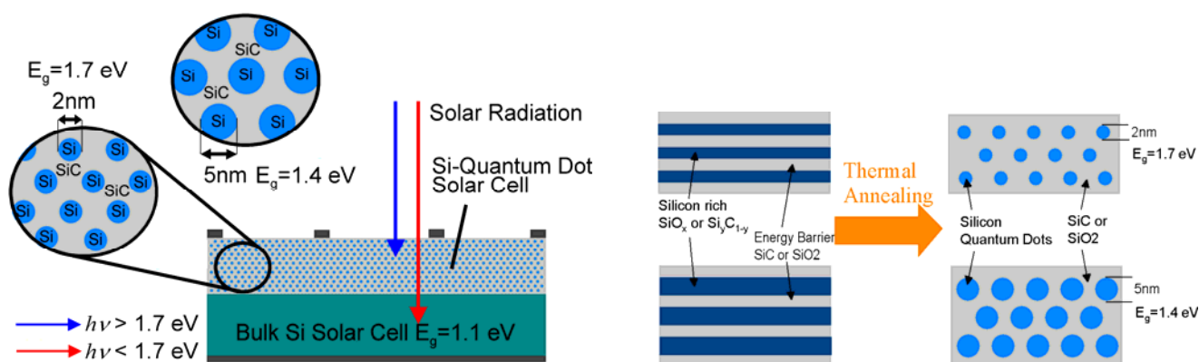
Figure 1: Principle of a crystalline Silicon tandem solar cell. The top solar cell consists of silicon nanocrystals in a silicon-based dielectric matrix such as \text{SiO}_2 , \text{Si}_3\text{N}_4 or \text{SiC} . The bandgap of the nanocrystal solar cell can be controlled by the nanocrystal size due to quantum confinement effects. The high band gap silicon compounds \text{SiO}_2 , \text{SiC} and \text{Si}_3\text{N}_4 are used as embedding matrices. All material systems are deposited as multilayers of alternating stoichiometric and Si rich layers. Si crystallites are formed in the Si rich layers by thermal annealing around 1100 °C. The stoichiometric layers act as diffusion barriers in the thermal annealing step and limit the size of the Si nanocrystals.
