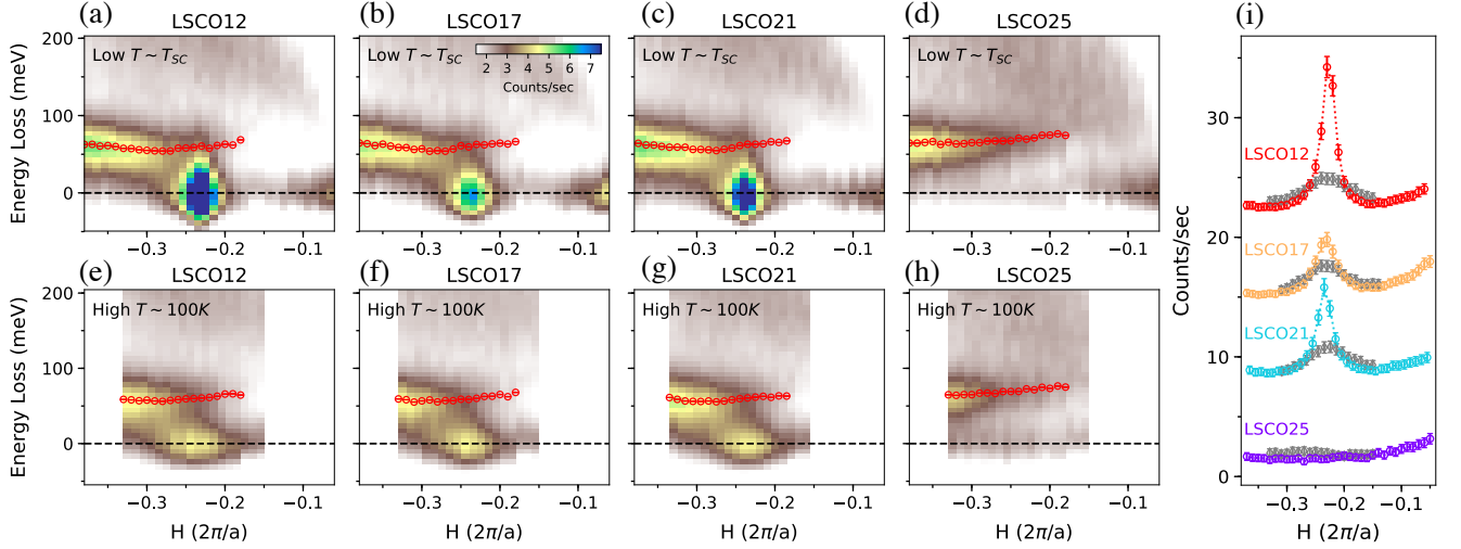
FIG. 2. Doping and temperature evolution. (a)-(d) show ( \Delta E = 55 meV) RIXS maps of \text{LSCO}_n ( n = 12, 17, 21, 25 ) at their superconducting transition temperature T_{\text{SC}} , where the CDW is strongest. All maps share the same colorscale inset in panel (b). Red circles represent the BS phonon energy. (e)-(h) The same measurement for T = 100 K. (i) Comparison of integrated intensity in the \pm 20 meV energy window. Data from panels (a)-(d) at T = T_{\text{SC}} are represented in color; data at T = 100 K from panels (e)-(h) are plotted in gray.
