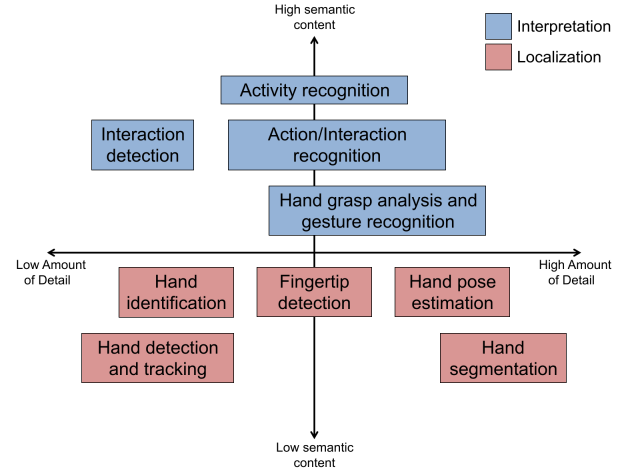
Fig. 1. Hand-based approaches in FPV categorized by amount of detail and semantic content.
