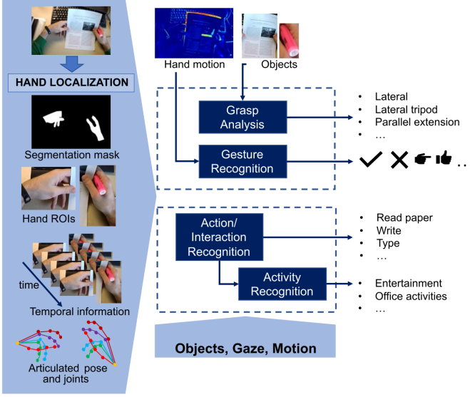
Fig. 3. Diagram of the hand interpretation areas in egocentric vision. Grasp analysis and gesture recognition focus directly on describing the hand. In action/interaction and activity recognition, the hand is instrumental in describing the user's behaviour.
