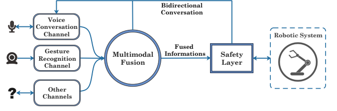
Fig. 1. Proposed Architecture
