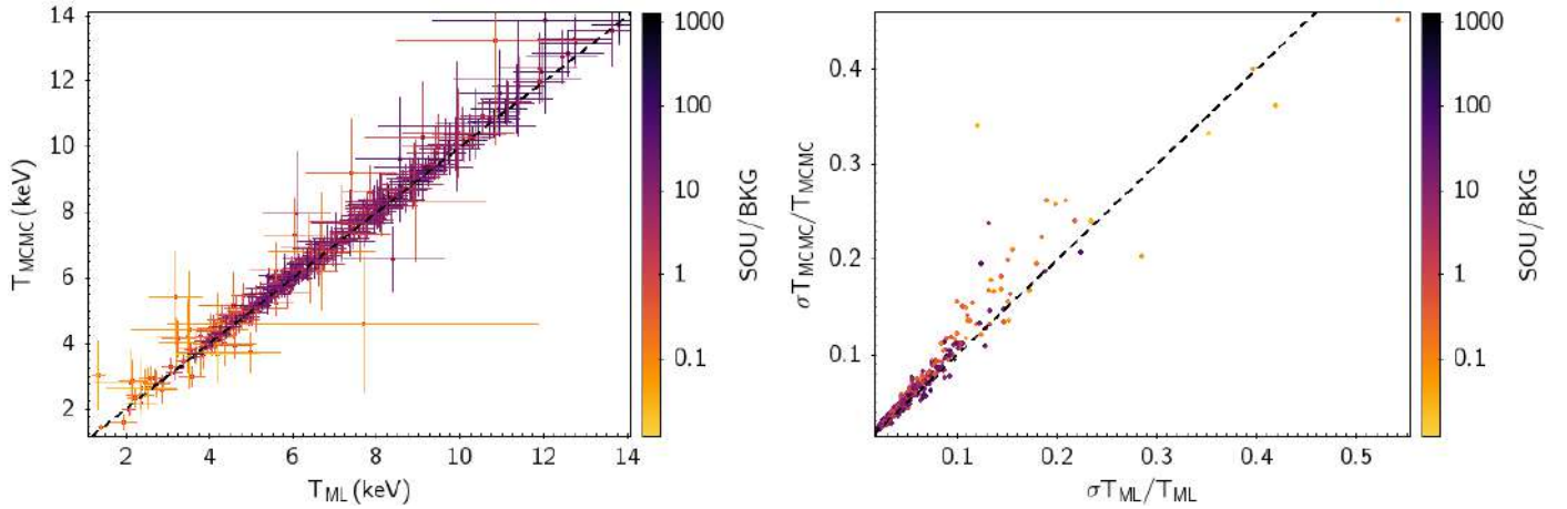
Fig. 6. Comparison of best-fit temperature values (left panel) and relative symmetric errors (right panel) for all clusters and all regions obtained with the standard ML technique (x-axis) and with the MCMC approach (y-axis). The color coding refers to the SOU/BKG ratio in each region, the dashed line represents the equality line.
