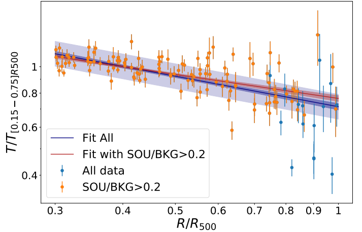
Fig. 17. Fit of the temperature profile with a power law for R > 0.3 R_{500} . Orange (blue) points represent regions where \text{SOU/BKG} is greater (smaller) than 0.2. The blue line and dark envelope represent the best fit function and its errors on the full dataset, while the light shaded area marks the intrinsic scatter. The red line and envelope show the best-fit for regions with \text{SOU/BKG} > 0.2 (intrinsic scatter not shown for clarity).
