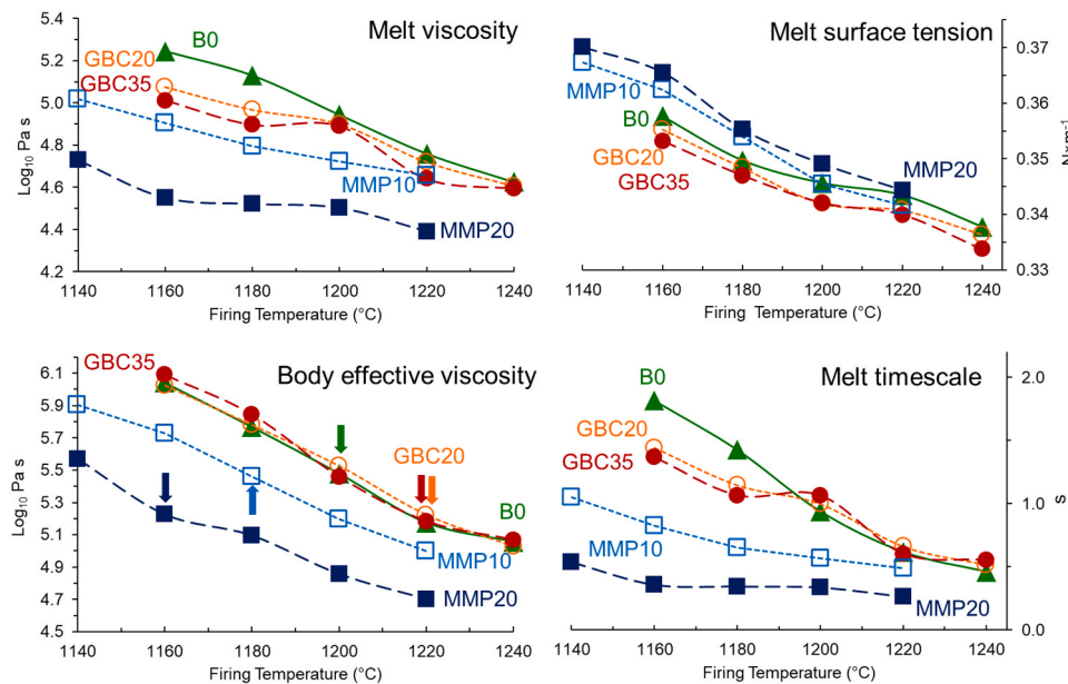
Fig. 8. Trends of calculated shear viscosity (Log 10 Pa·s), surface tension (N·m -1 ) and timescale (s) of the melt, and effective viscosity of the bulk (Log 10 Pa·s) as a function of firing temperature (°C). Arrows indicate the temperature of maximum densification for each batch. Experimental error is within the symbol size.
