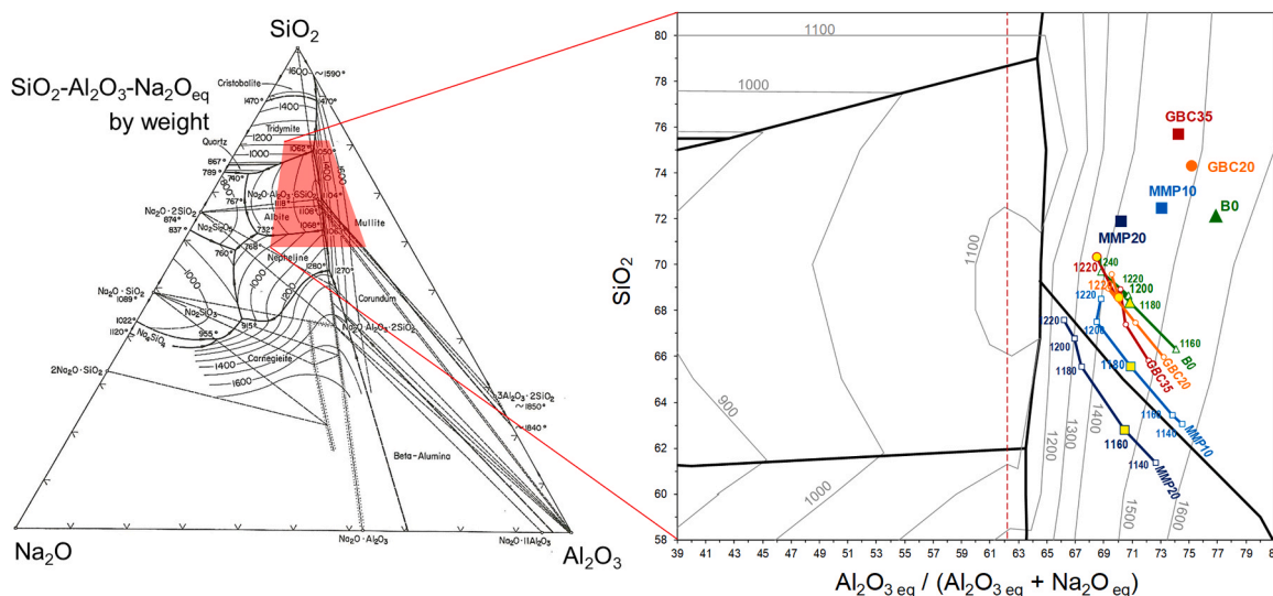
Fig. 4. Aluminosity-silica diagram with batch compositions (full symbols) and vitrification paths (melt composition at different temperatures) with maximum densification highlighted. For the diagram construction, see Conte et al. [67].
