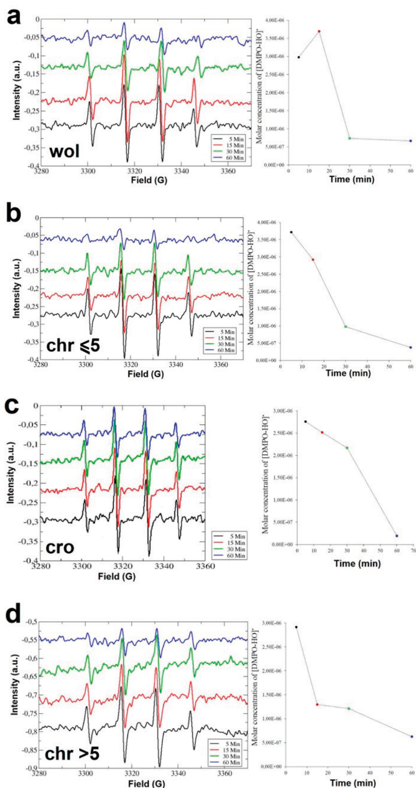
Figure 6. EPR spectra of [DMPO-OH] ^{\bullet} adduct and quantitative plot of (A) wol= NYAD G wollastonite; (B) chr \leq 5 =Russian short ( \leq 5 mm) chrysotile fibres; (C) cro=UICC crocidolite; (D) chr > 5 =Russian long ( > 5 \mu m) chrysotile fibres.
