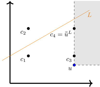
Figure 7: The double bar of u with respect to the line L is the value c_4 \in \overline{C} . In this case we also have \bar{c}_3^L = \bar{u}^L = c_4 .
