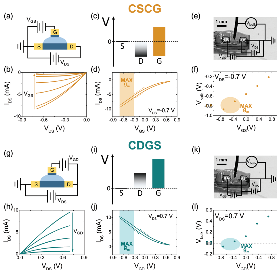
Figure 1. Benchside comparison of EGOT configuration. a) Connection layout of the common-source/common-ground (CSCG) EGOT. b) I - V output characteristics recorded in CSCG configuration scanning V_{DS} from -0.7 to 0.0 V at fixed V_{GS} values ranging from -0.7 to 0.7 V. Arrow indicates increasing V_{GS} . c) Schematic representation of the spans of the driving voltages in CSCG configuration. d) I - V transfer characteristic recorded in CSCG configuration scanning V_{GS} from -0.7 to 0.7 V at V_{DS} = -0.7 V. The maximum transconductance regime is highlighted. e) Photograph and circuit schematics of the V_{bulk} recording setup for CSCG EGOT. f) Scatter plot showing the dependence of V_{bulk} on V_{GS} in CSCG configuration, with highlighted maximum transconductance regime, showing strong negative V_{bulk} values at maximum transconductance. g) Connection layout of the common-drain/grounded-source (CDGS) EGOT. h) I - V output characteristics recorded in CDGS configuration scanning V_{DS} from 0.0 to 0.7 V at fixed V_{GD} values ranging from -0.7 to 0.7 V. Arrow indicates increasing V_{GD} . i) Schematic representation of the spans of the driving voltages in CDGS configuration. j) I - V transfer characteristic recorded in CDGS configuration scanning V_{GD} from -0.7 to 0.7 V at V_{DS} = 0.7 V. The maximum transconductance regime is highlighted. k) Photograph and circuit schematics of the V_{bulk} recording setup for CDGS EGOT. l) Scatter plot showing the dependence of V_{bulk} on V_{GD} in CDGS configuration, with highlighted maximum transconductance regime, showing null V_{bulk} at maximum transconductance.
