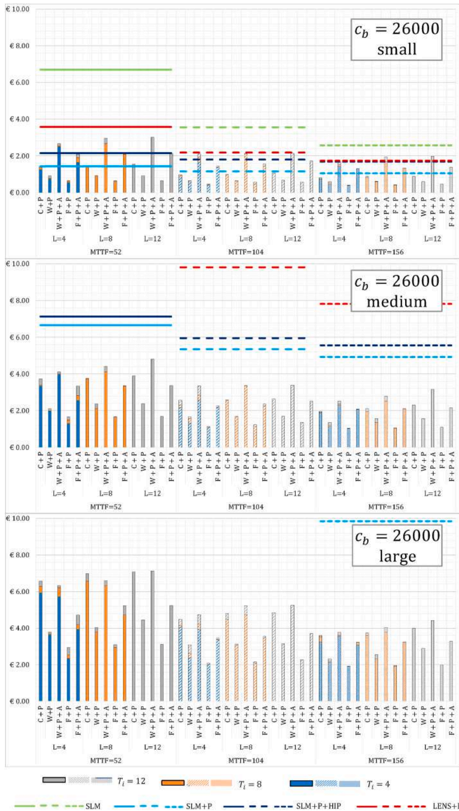
Fig. 4. Spare parts inventory management costs for different part size and reliability and of different CM review periods and procurement lead times considering the entire data set for MTTF ratio. c_b is 26000 €/unit.
