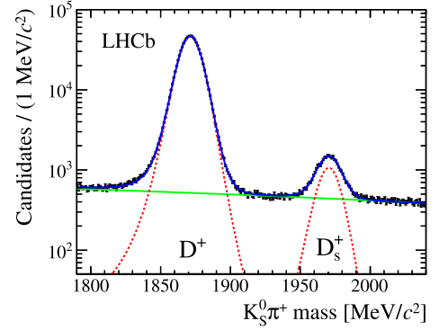
Fig. 1. Mass distribution of selected K_S^0 \pi^+ candidates. The data are represented by symbols with error bars. The dashed curves indicate the signal and the D_s^+ \rightarrow K_S^0 \pi^+ decays, the lower solid line represents the background shape, and the upper solid line shows the sum of all fit components.
