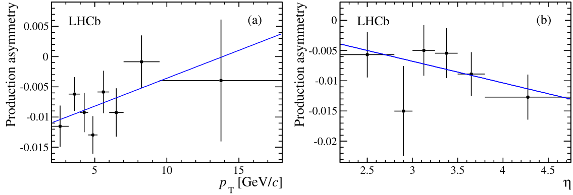
Fig. 4. Production asymmetry as a function of (a) transverse momentum p_T and (b) pseudorapidity \eta . The straight line fits have slopes of (0.09 \pm 0.07) \times 10^{-2} \text{ (GeV/c)}^{-1} and (-0.36 \pm 0.28)\% , and values of \chi^2 per degree of freedom of 5.5/6 and 2.2/4, respectively. The error bars include only the statistical uncertainty on the D^+ signal sample and are uncorrelated within a given plot.
