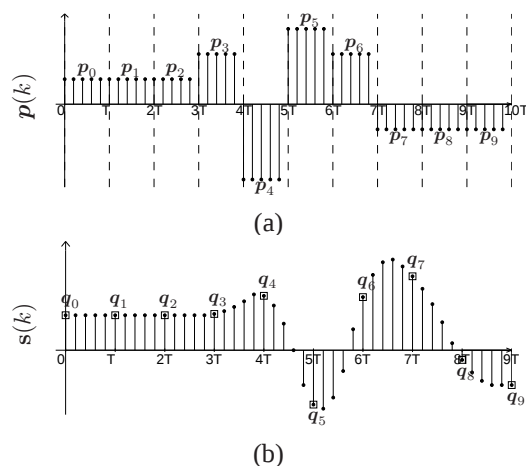
Fig. 1. Piecewise constant sequence p(k) (a) generating the discrete-time spline s(k) that interpolates the given points q_j (b).
