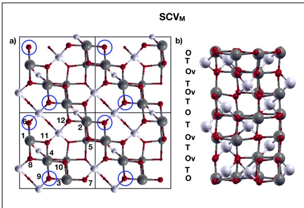
Fig. 3 a) Top view of the (2 \times 2) unit cell of the SCV_M reconstruction of the \gamma\text{-Fe}_2\text{O}_3 (001) surface; b) side view of the slab used to model the SVC_M reconstruction of the \gamma\text{-Fe}_2\text{O}_3 (001) surface. The color code is the same as in Fig. 2. Blue circles indicate the location of the Fe vacancy in the third layer below the outermost plane. The numbers label the atoms on the outermost layer as explained in the text.
