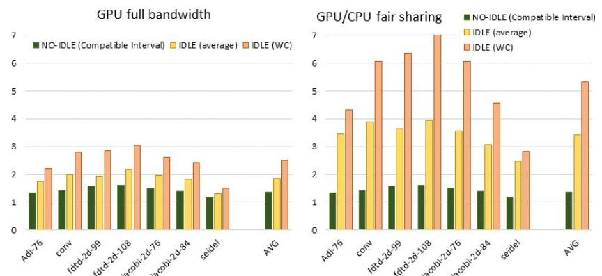
Fig. 5: Idle time introduced when budgeting for the worst case and average timer latencies under two different system memory schedules.
