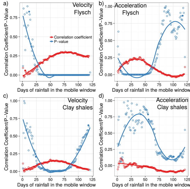
Figure 8: Correlation coefficients and P-values for the relationships between a) velocity and rainfall and b) acceleration on landslides in pelitic flysch formations and different days of preceding rainfall added to the daily rainfall values. c) Correlation coefficients and P-values for the relationship between velocity and d) acceleration on landslides in chaotic clay shales.
