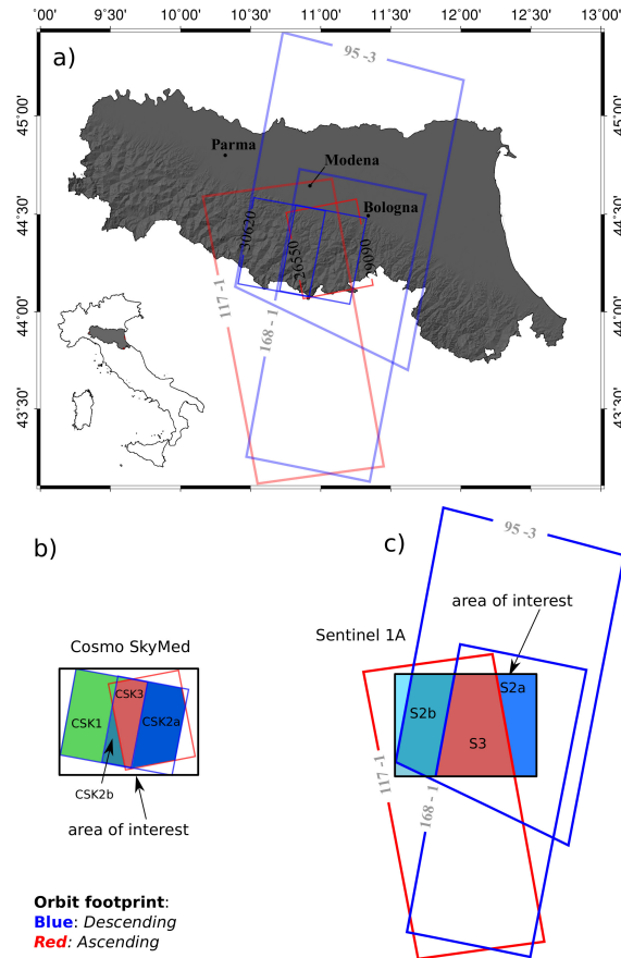
Figure 2: a) The area of interest is located in the Northern Apennines of Italy and is covered by several SAR frames in both ascending and descending viewing geometries. b) For COSMO SkyMed one ascending and two descending swaths were available. A small area is covered by all three datasets (CSK3), while most parts of our study area are covered by either two (CSK2a and CSK2b) or one dataset (CSK1). c) Also for Sentinel 1A one ascending and two descending tracks were processed, which results in a larger area covered by either two (S2a and S2b) or three InSAR datasets (S3). Details regarding the different datasets and their combination can be found in Tab. 1.
