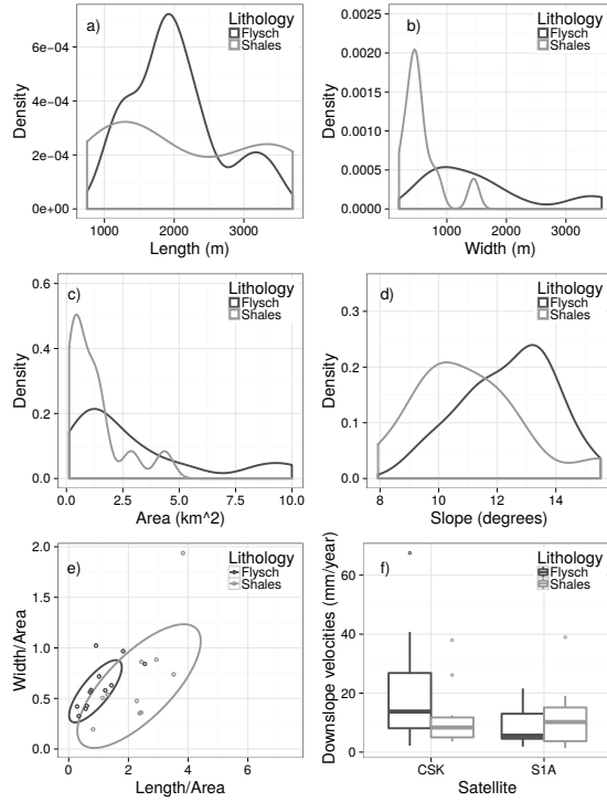
Figure 4: Probability density distributions calculated with a gaussian kernel of a) landslide lengths, b) widths, c) area, d) slope angles and e) the relationship between width and length, normalized by the landslide area for InSAR detectable landslides in our study area for the two main lithologies. f) 75 percentile of the mean downslope velocities measured on the landslides in pelitic flysch formations and chaotic clay shales.
