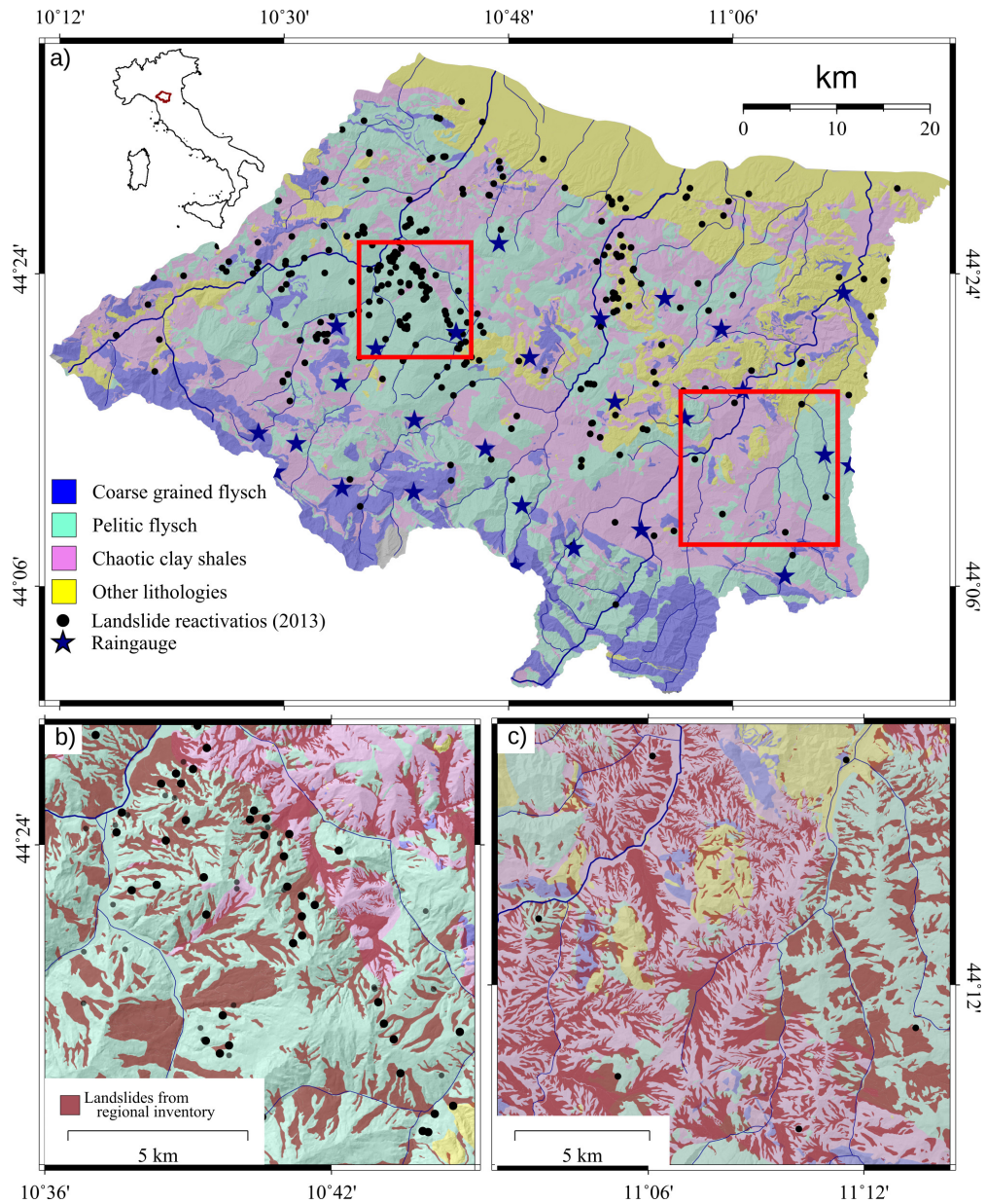
Fig. 1: a) Lithological map of the study area (Berti et al., 2012) with the reactivations that were registered by the regional authorities during spring 2013 and the raingauges that are available in the study area. b) Lithological map with landslide perimeters over the western part of the study area, where pelitic flysch formations crop out more extensively compared to c) the eastern part of the study area, where chaotic clay shales are more common. The landslide perimeters area derived from a detailed regional inventory (Servizio Geologico, Sismico e dei Suoli della Regione Emilia-Romagna, 2014) and In Fig. 1 of the supplementary I we report the main statistical aspects of this landslide inventory, the reactivations and the annual rainfall derived from the raingauges pattern in the study area.
