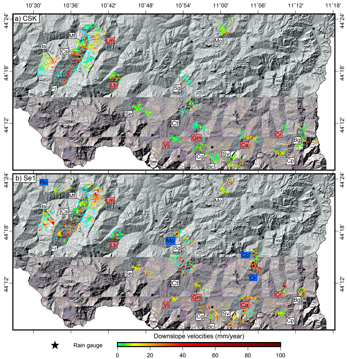
Figure 3: a) Calibrated InSAR results for all landslides that caused a clear deformation signal in the COSMO SkyMed datasets. Black stars indicate rain gauges that were used to retrieve regional rainfall that will be discussed together with displacement signals in section 4.2. b) Calibrated InSAR results for Sentinel 1A. The labels in a) and b) are localities, where distinct landslides were detected. From West to East and from South to North we have: Bs: Boschi di Valoria, Fr: Frassinoro, Cs: Casolare, Ro: Roncolo, Mf: Montefiorino, Lm: Lama di Monchio, Lb: La Borra, Se: Sestola, Vi: Vidiciatico, Sg: San Giacomo, Gm: Gaggio Montano, Ct: Castelluccio, Bc: Borgo Cappanne Mo: Monte Ombraro, Sv: Suviana, Ca: Camugnano, Cp: Castiglione dei Pepoli, Cr: Creda, Bg: Il Borgo. Red highlighted labels indicate selected landslide cases that are discussed in detail in section 5. Blue labels are cases that were only visible in the Sentinel dataset.
