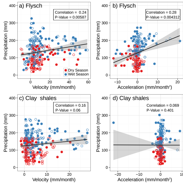
Figure 9: a) Relationship between velocity on landslides in pelitic flysch and rainfall if 40 days of preceding rainfall are summed to the daily values. b) Relationship between acceleration and rainfall on pelitic flysch landslides. c) Comparison between velocity and d) acceleration of landslides in chaotic clay shales and rainfall.
