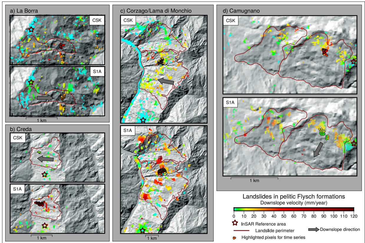
Figure 5: Deformation maps for selected rockslides in pelitic flysch formations. CSK and Se1 results a) at La Borra, b) at Creda, c) at Corzago/Lama di Monchio, d) at Camugnano. Due to the high spatial resolution, the number of registered pixels are higher for COSMO SkyMed, yet Sentinel selects also points in areas, where COSMO SkyMed was decorrelated. Displacement patterns vary in space for the different periods and the highlighted pixels were used to produce the time series in Fig. 7 a) and d)
