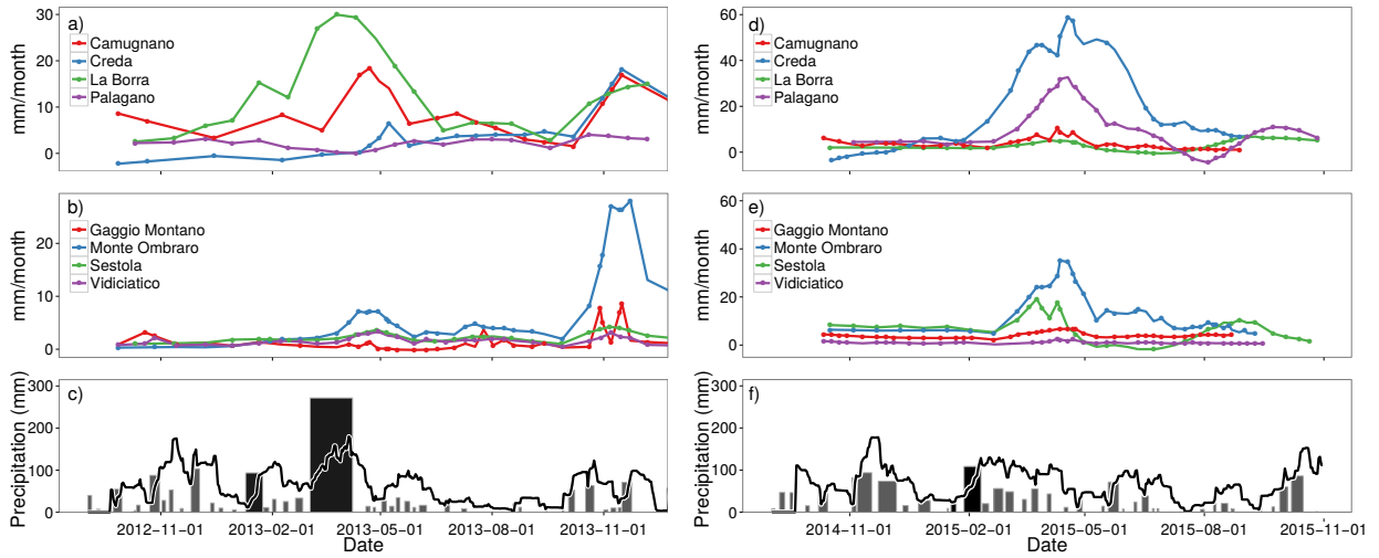
Figure 7: a) Velocity time series for landslides in pelitic flysch during for the year 2013. b) Velocity time series for earthflows in the chaotic clay shales for 2013. c) The grey bars are rainfall events that were defined by the methodology proposed by Berti et al. (2012), while the black line depicts daily rainfall that takes into account the preceding 20 days of rainfall. We chose 20 days because this timespan is in good agreement with our definition of rainfall events. d) Displacement rates derived from Sentinel for the year 2015 on rockslides in pelitic flysch. e) Velocity time series for earthflows in mélangé type rocks. f) Daily rainfall that takes into account the preceding 20 days and it is plotted together with rainfall events for the year 2015.
