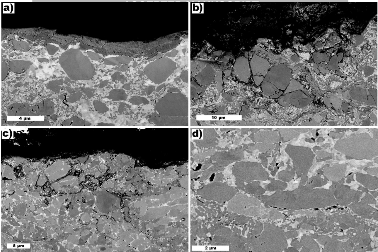
Figure 16: SEM micrograph of the wear track cross section of a) HVOF and b) HVOF sprayed \text{Cr}_3\text{C}_2\text{-}25\text{NiCr} coatings, and of c) HVOF sprayed \text{Cr}_3\text{C}_2\text{-}25\text{NiCr} coating from plasma densified powder, with d) detail of secondary carbides precipitation within the NiCr matrix.
