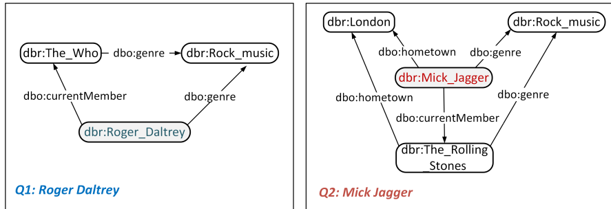
Figure 3: A portion of the Contextual Graph extracted from DBpedia for the two keyword queries: Roger Daltrey and Mick Jagger
