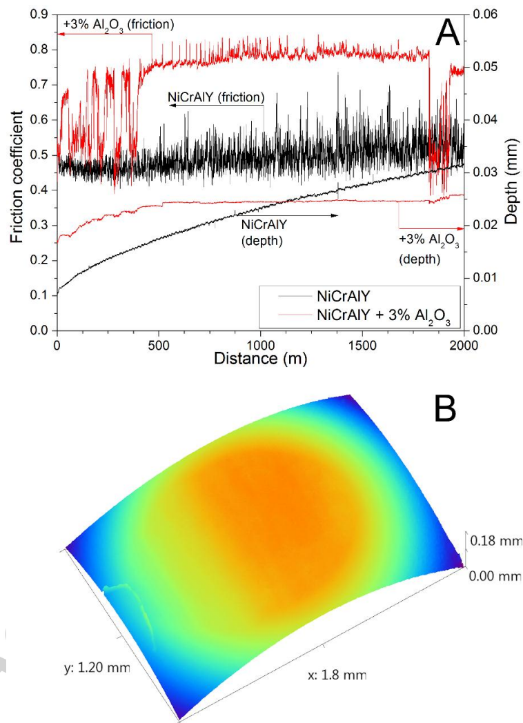
Figure 13. Evolution of the friction coefficient and of the overall wear depth recorded during room-temperature ball-on-disk wear tests on the NiCrAlY and NiCrAlY+3 Al 2 O 3 samples (A) and 3D profile of the worn surface of the counterpart tested against the NiCrAlY sample at room temperature, after removal of the transfer layer (B).
