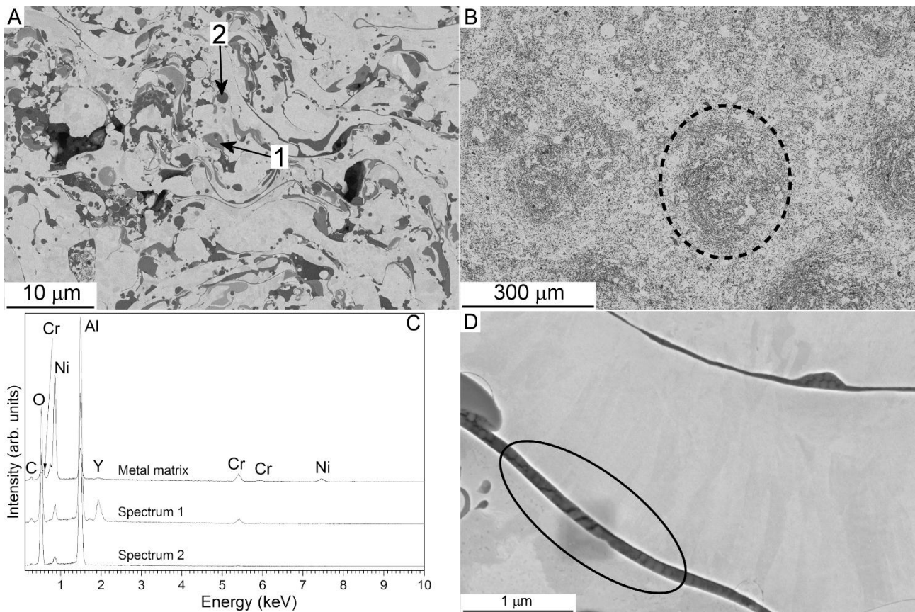
Figure 3. Backscattered electron FEG-SEM micrographs of the cross-section of the NiCrAlY + 3 wt.% Al 2 O 3 sample (A) and of the polished top surface (B) of the NiCrAlY + 18 wt.% Al 2 O 3 sample, with EDX microanalysis (C) of the areas indicated in panel A. Detail of a microcracked oxide inclusion (circled area) along the boundary between adjacent NiCrAlY lamellae in the NiCrAlY + 6 wt.% Al 2 O 3 coating (D).
